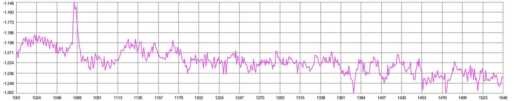
67 V1G1 - 70 V1G4 Easting Mean: -1.222m Min: -1.262 Max: -1.148 SD: 0.015
