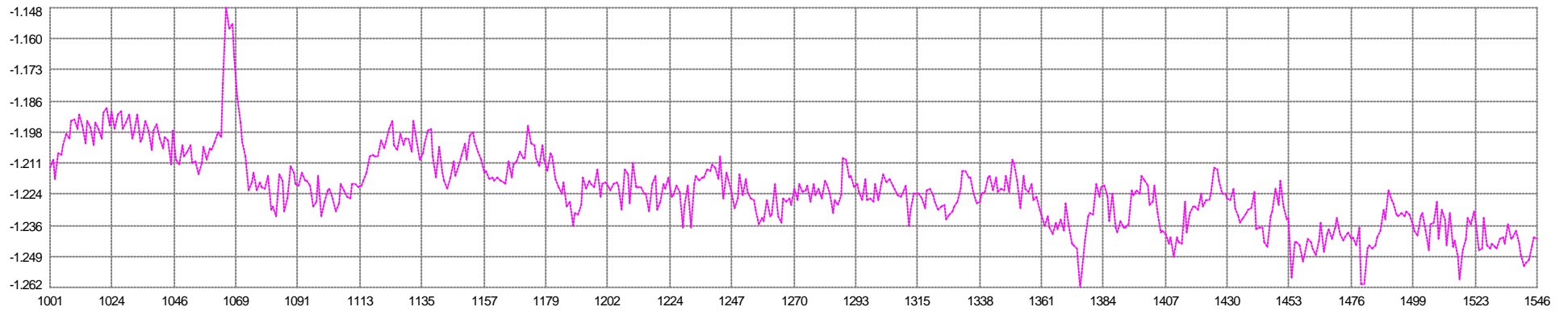
67 V1G1 - 69 V1G3 ■ Easting Mean: -1.222m Min: -1.262 Max: -1.148 SD: 0.015
