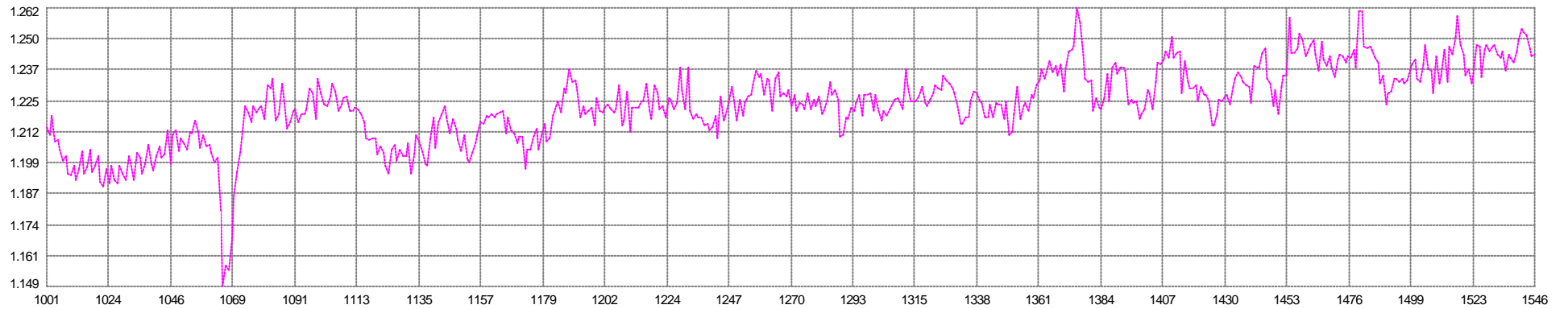
68 V1G2 - 71 V1G5 Easting Mean: 1.223m Min: 1.149 Max: 1.262 SD: 0.016
