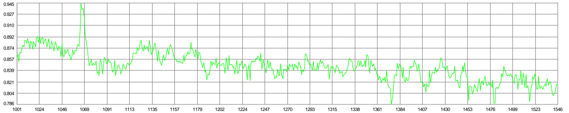
68 V1G2 - 71 V1G5 ■ Northing Mean: 0.846m Min: 0.786 Max: 0.945 SD: 0.022
