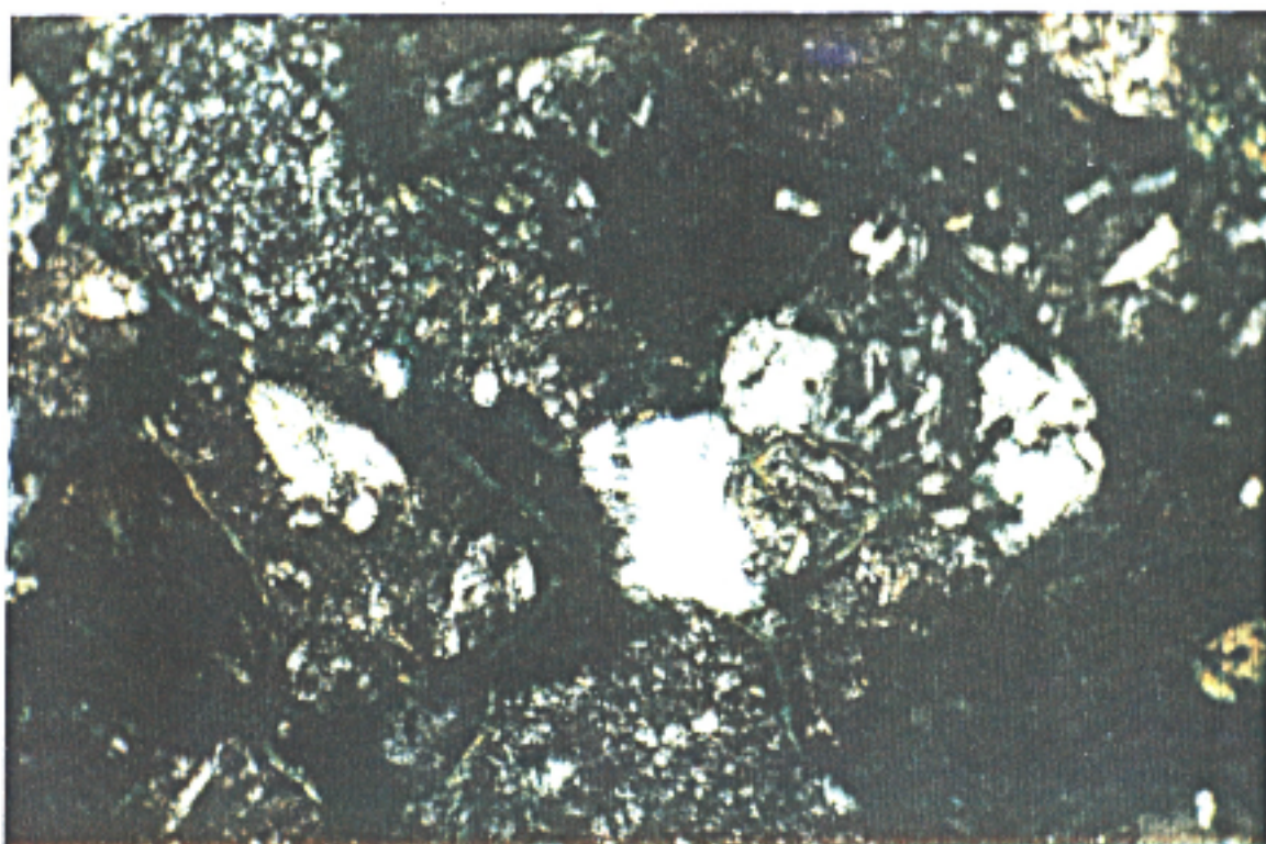
PHOTO 6 1806.3M VOLCANIC CLASTS IN LITHIC TUFF, PLUS CHLORITE RIM. NIC CROS. FIELD WIDTH 1.8MM
