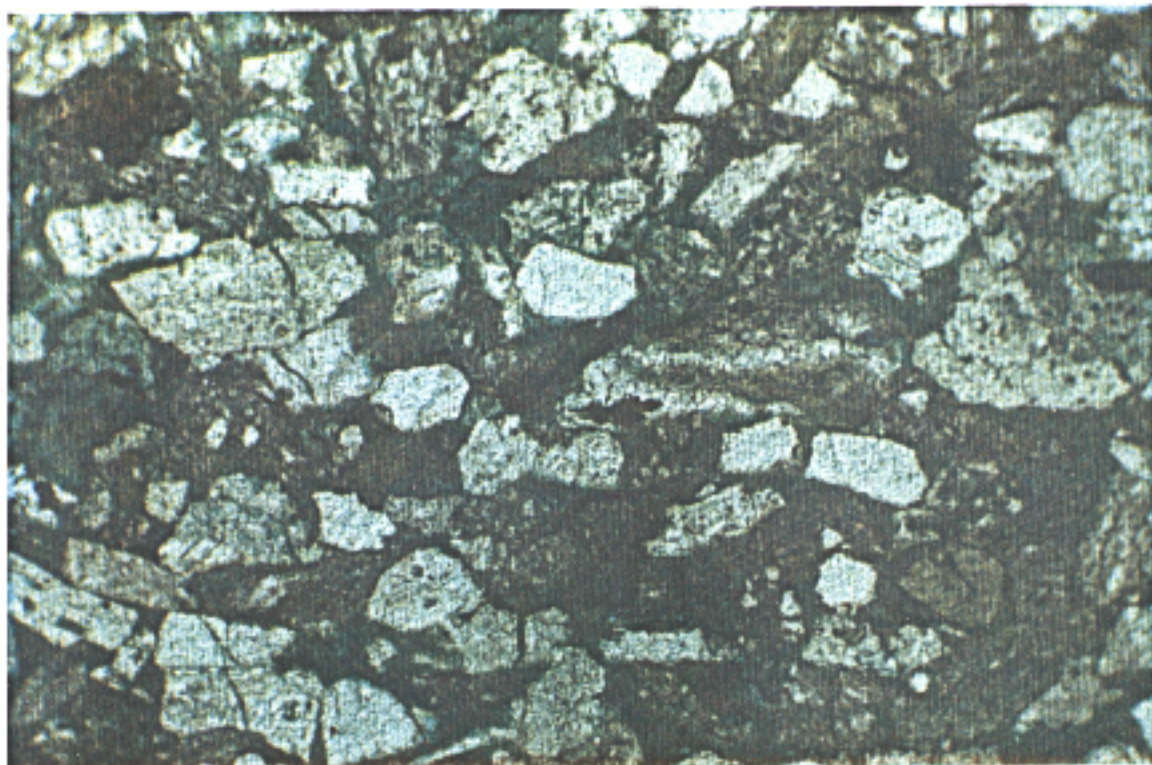
PHOTO 5 1806.3M WELL SORTED LITHIC CRYSTAL TUFF, SHOWING SLIGHT ALIGNMENT OF CLASTS. NIC UNC. FIELD WIDTH 1.8MM
