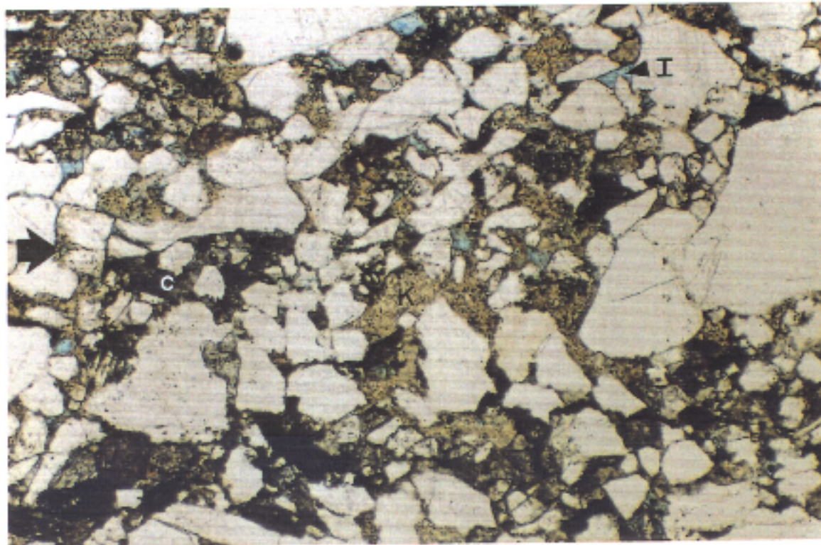
Figure 1a. Thin section photomicrograph illustrating porosity occlusion by kaolin (K) and carbonate (C). Intergranular (I) and dissolution (arrow) porosity are evident. Warracbarunah #5, Sample 1, core 15, depth 1524.88-1527.46m. Plane light. Field of view 2.72mm
