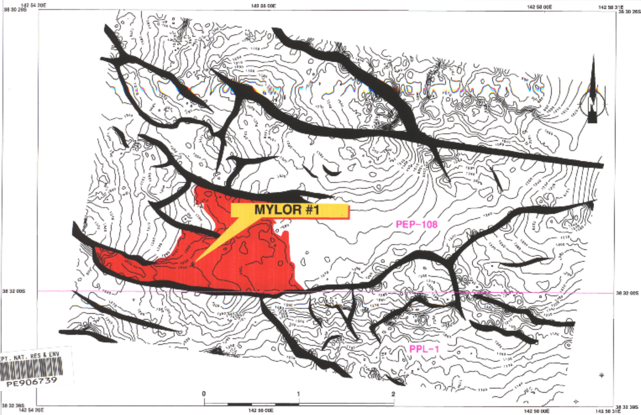
TWT STRUCTURE CONTOUR MAP ON THE TOP WAARRE FORMATION
