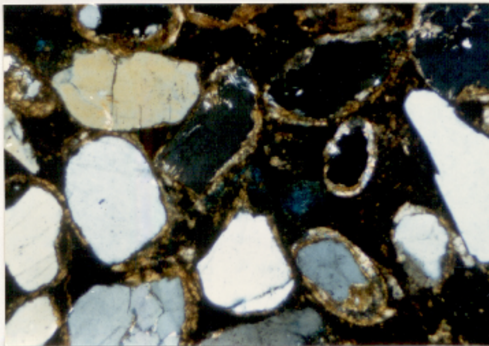
FIGURE 6 (a and b): Henke-1, SWC 9. PPL (a) and crossed Nicols (b), 2 mm. Typical field. Grains show a mantle of carbonate of several stages whereas most intergranular space is occupied by iron stained clay. Porosity (blue) is probably of secondary origin.
