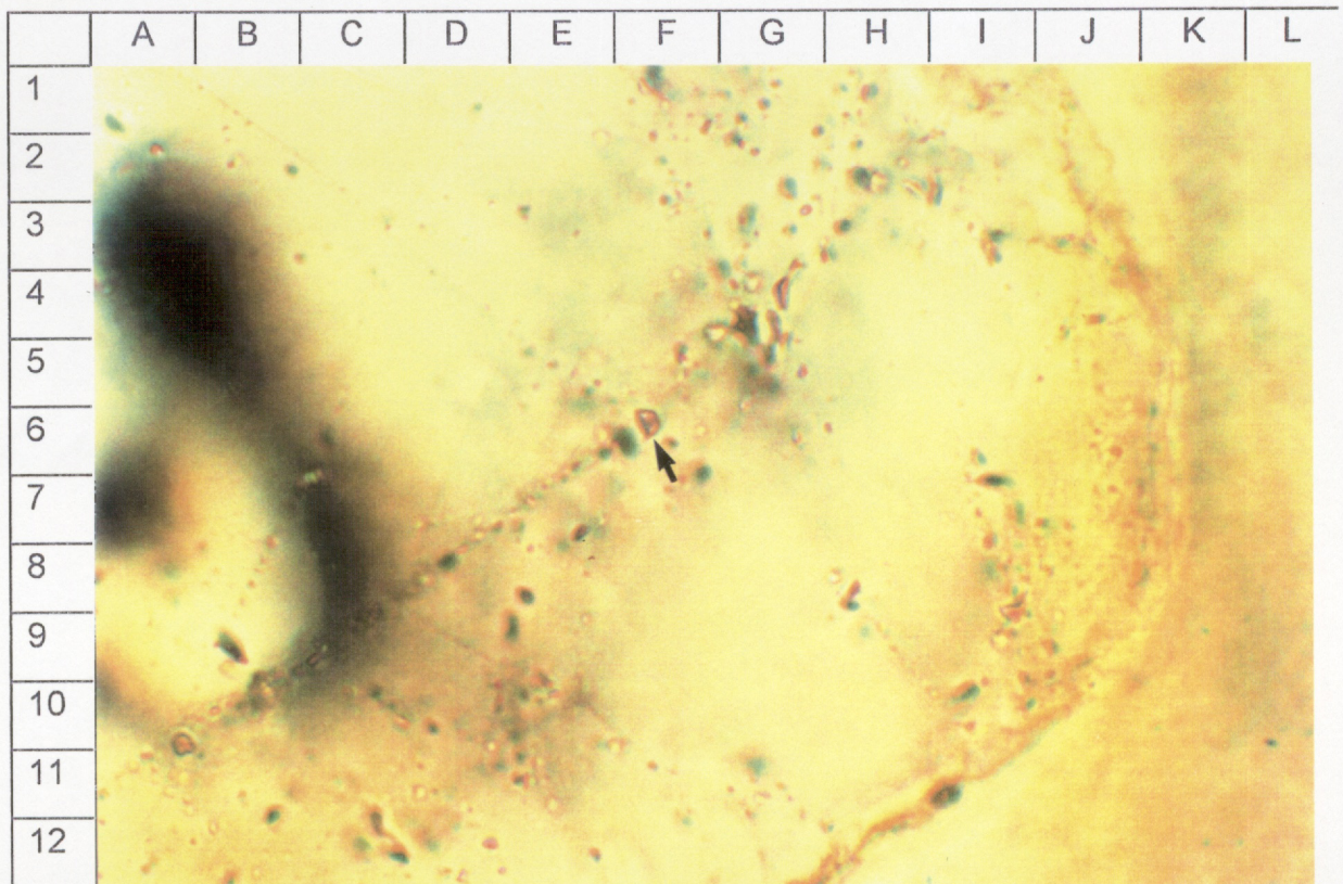
Figure 7B Same subject as 7A in transmitted light. The inclusion comprises a liquid phase and a small shrinkage bubble which develops in response to changes in temperature and pressure during sample retrieval. (10 \mu\text{m} = 17.5 mm).
