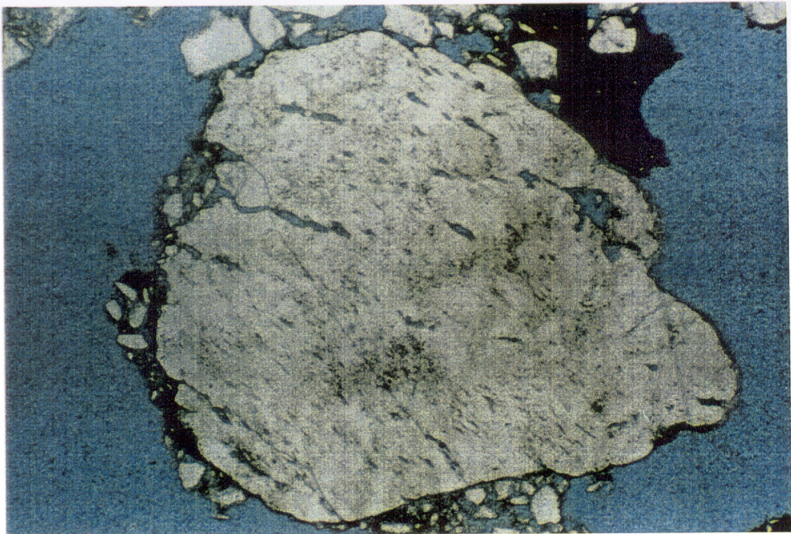
Figure 24. Thin section photomicrograph of secondary dissolution porosity in feldspar. Mudskipper #1, depth 1503.5m. Plane light. Field of view 2.40mm.
