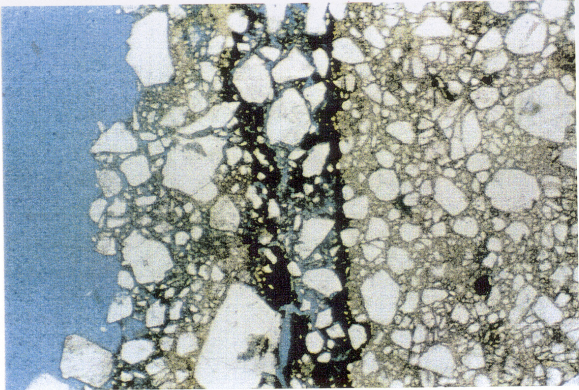
Figure 23. Thin section photomicrograph of a channel lined by iron oxide in quartzarenite. Mudskipper #1, depth 1503.5m. Plane light. Field of view 2.72mm.
