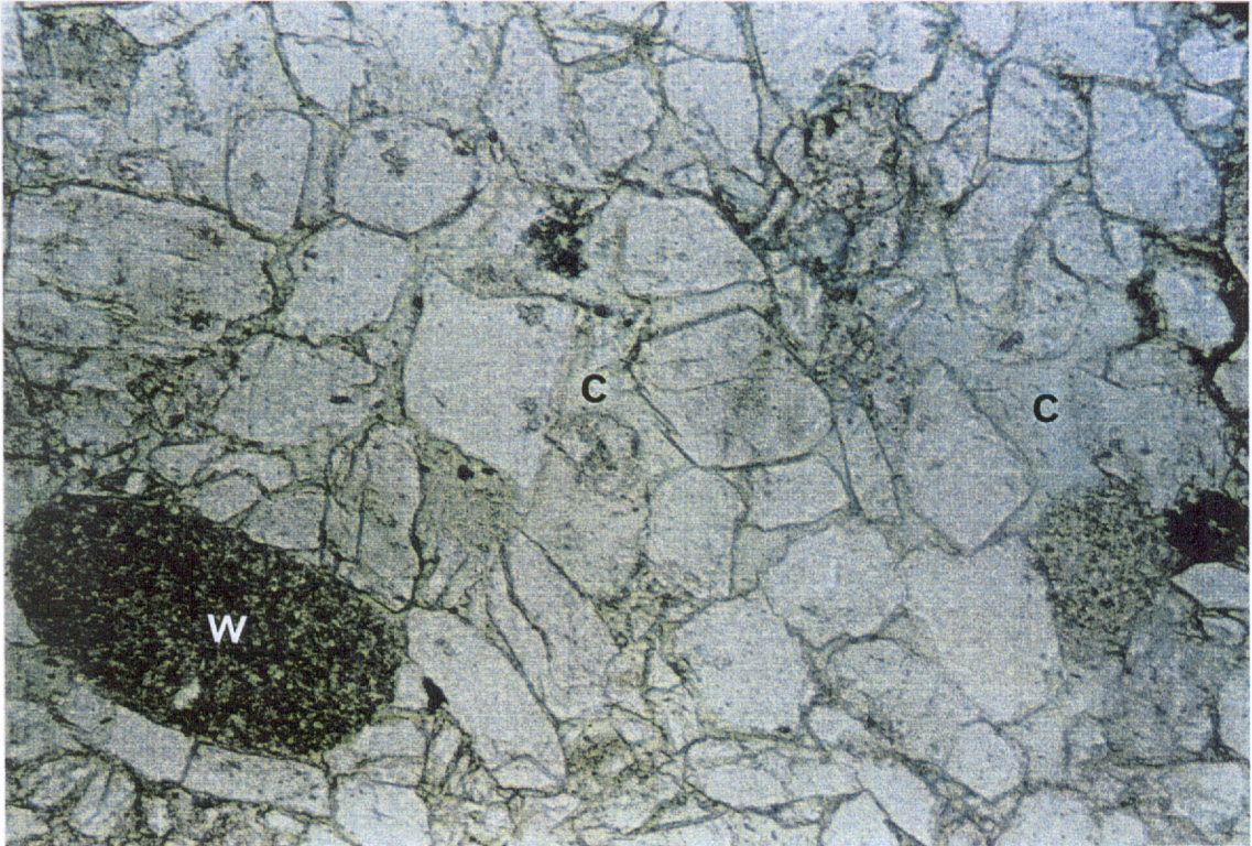
Figure 13a. Thin section photomicrograph of quartzarenite with pore spaces occluded by chlorite (C). Well rounded lithics (W) are rare. Mudskipper #1, depth 1590.5m. Plane light. Field of view 0.88mm.
