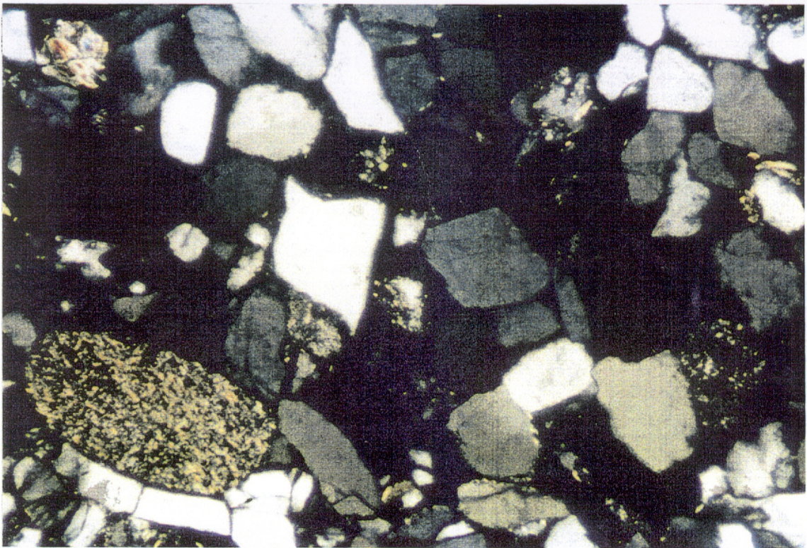
Figure 13b. Same field of view as Figure 13a in crossed nicols. Well rounded lithic is micaceous.
