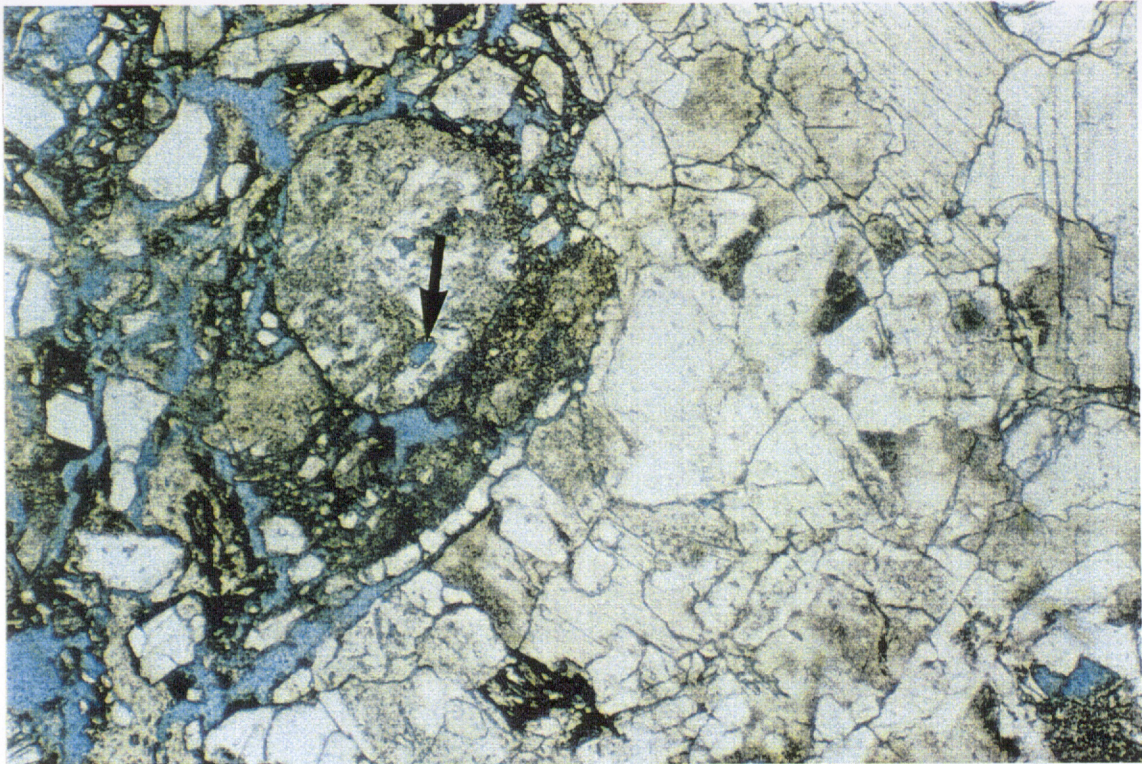
Figure 1a. Thin section photomicrograph of granular granite. The sample is highly disturbed with trace amounts of secondary dissolution pores (arrow). Mudskipper #1, depth 1615.0m. Plane light. Field of view 2.40mm.
