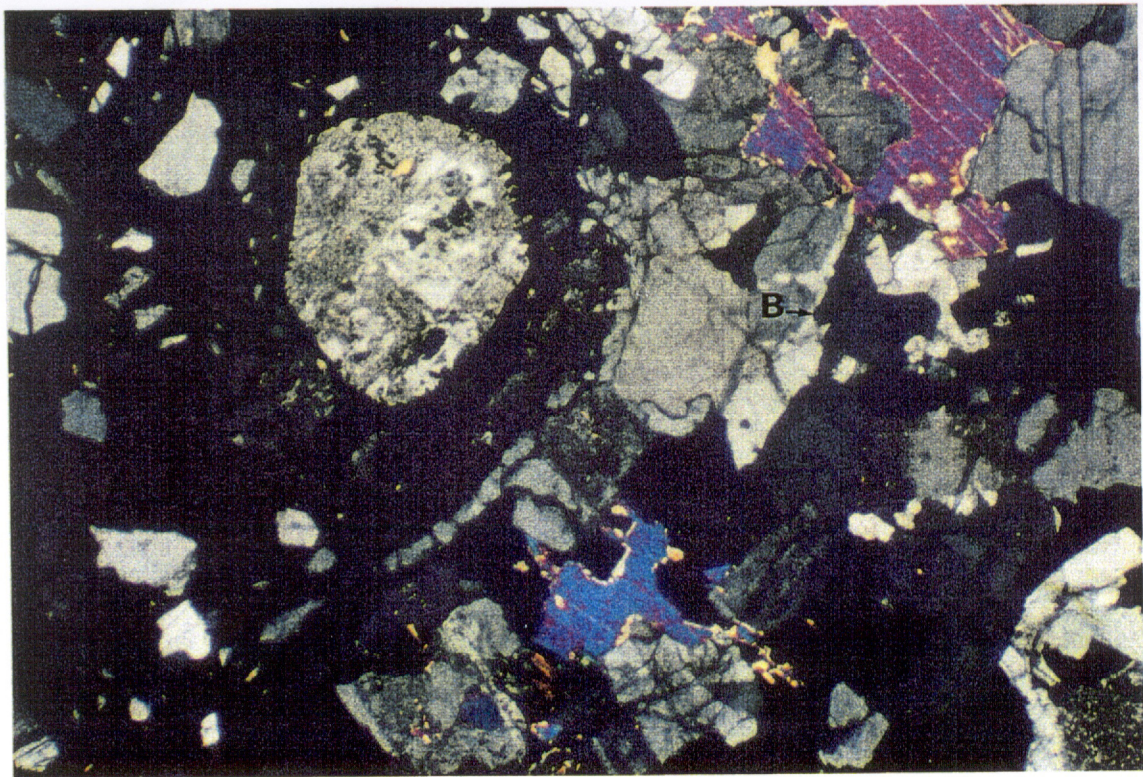
Figure 1b. Same field of view as Figure 1a in crossed nicols. Slightly interdigitating boundaries (B) indicate a consertal texture.
