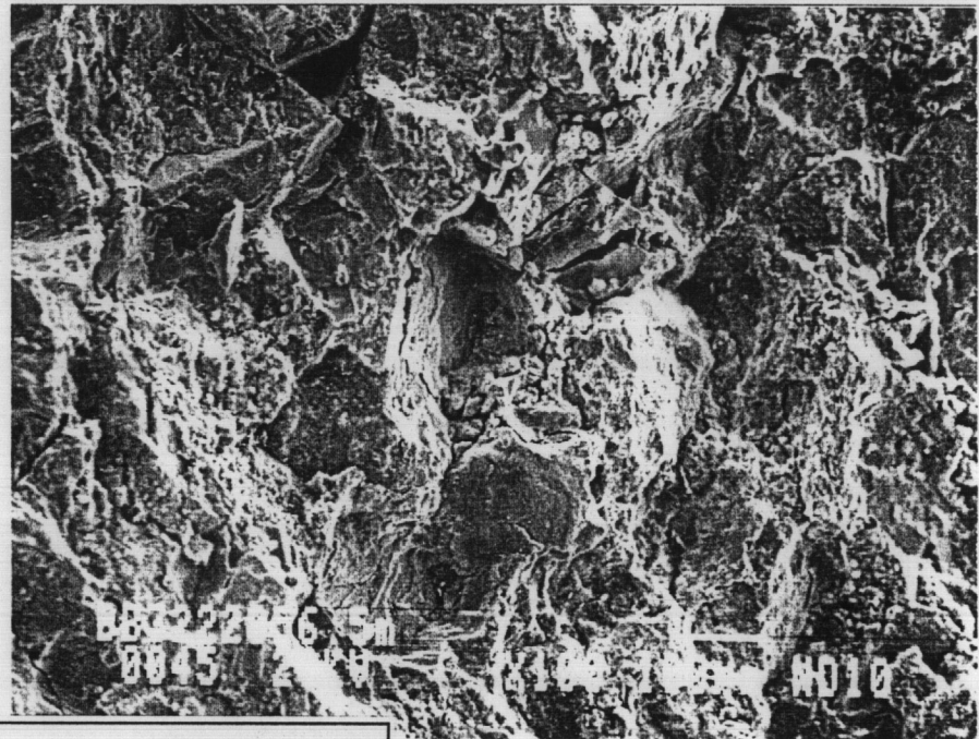
Figure 3B Blackback 3 2856.5m (plug 22) SEM x 50, x 100, x 600: diagenetic clays have large impact on porosity reduction.
