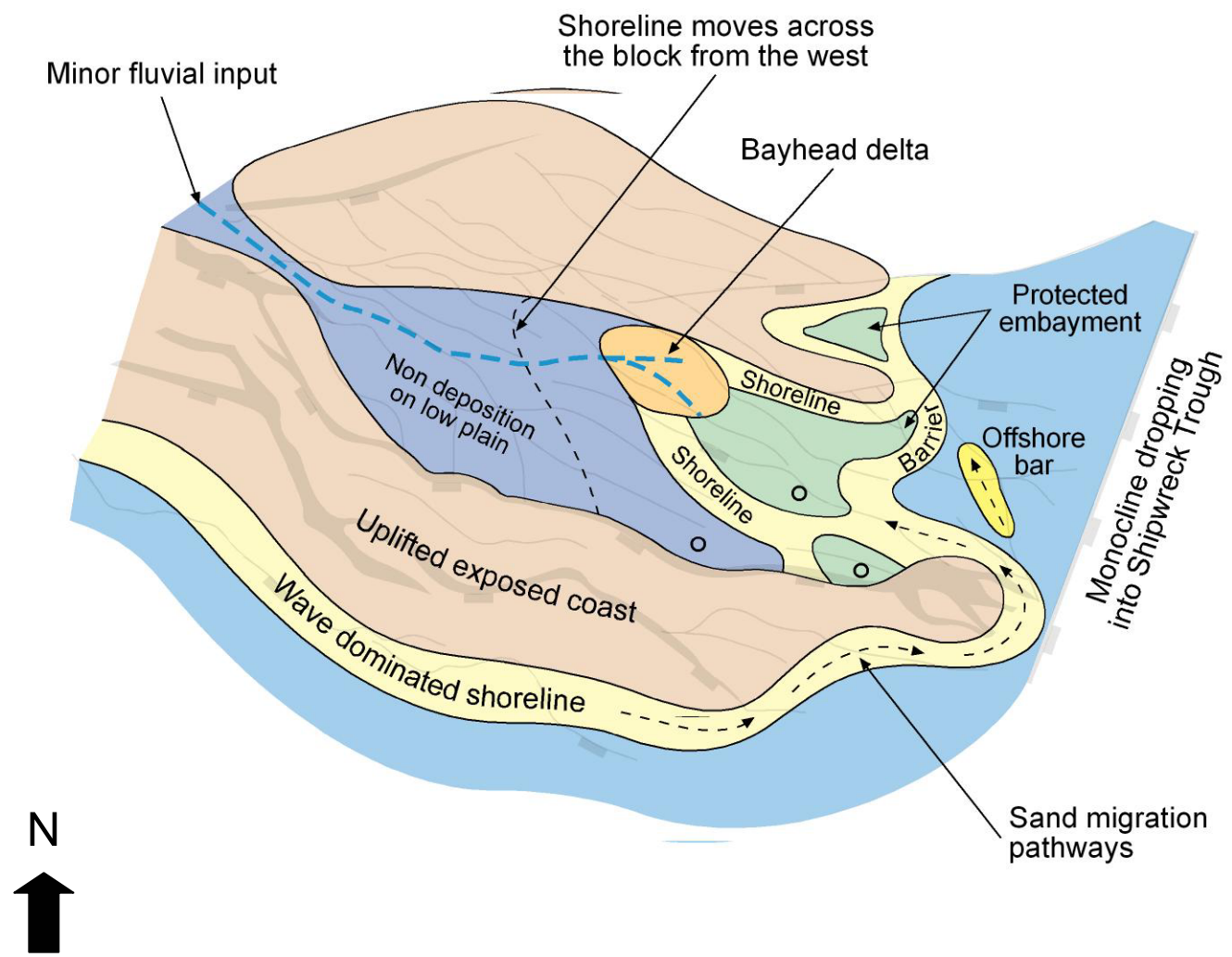
Facies on the Casino Block shown at the shoreline position currently defined by the truncation edge of the Waarre Ca interval between C1 and C2. Snapshot at time of Upper Waarre Ca.
