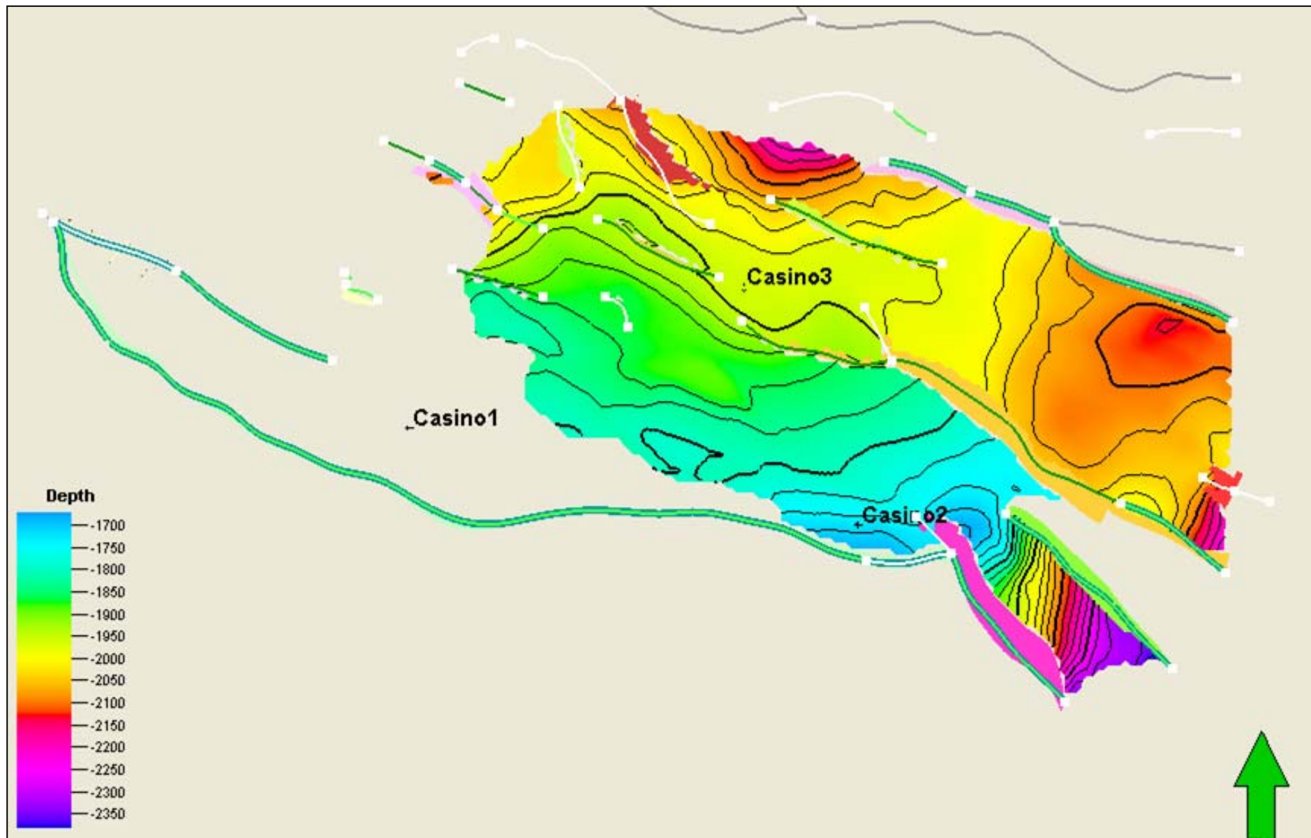
Figure 3.3.3-c: Top Waarre C low impedance depth map
