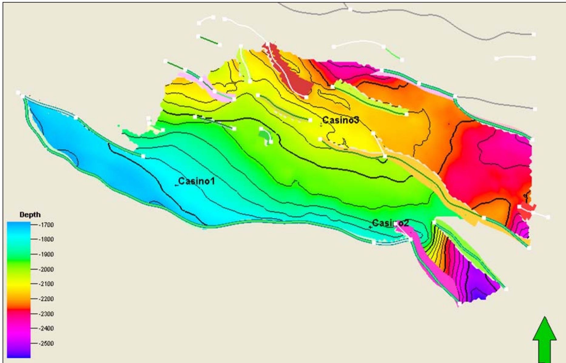
Figure 3.3.3-g: Base Waarre A depth map
