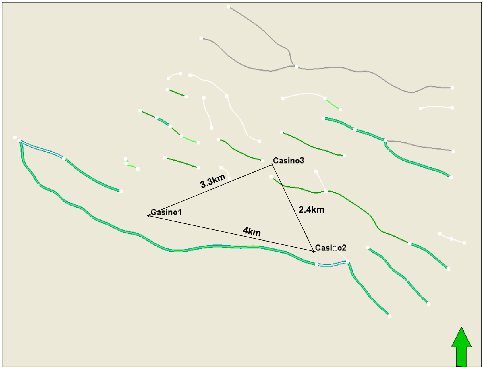
Figure 3.3.5-a: Petrel model fault map
