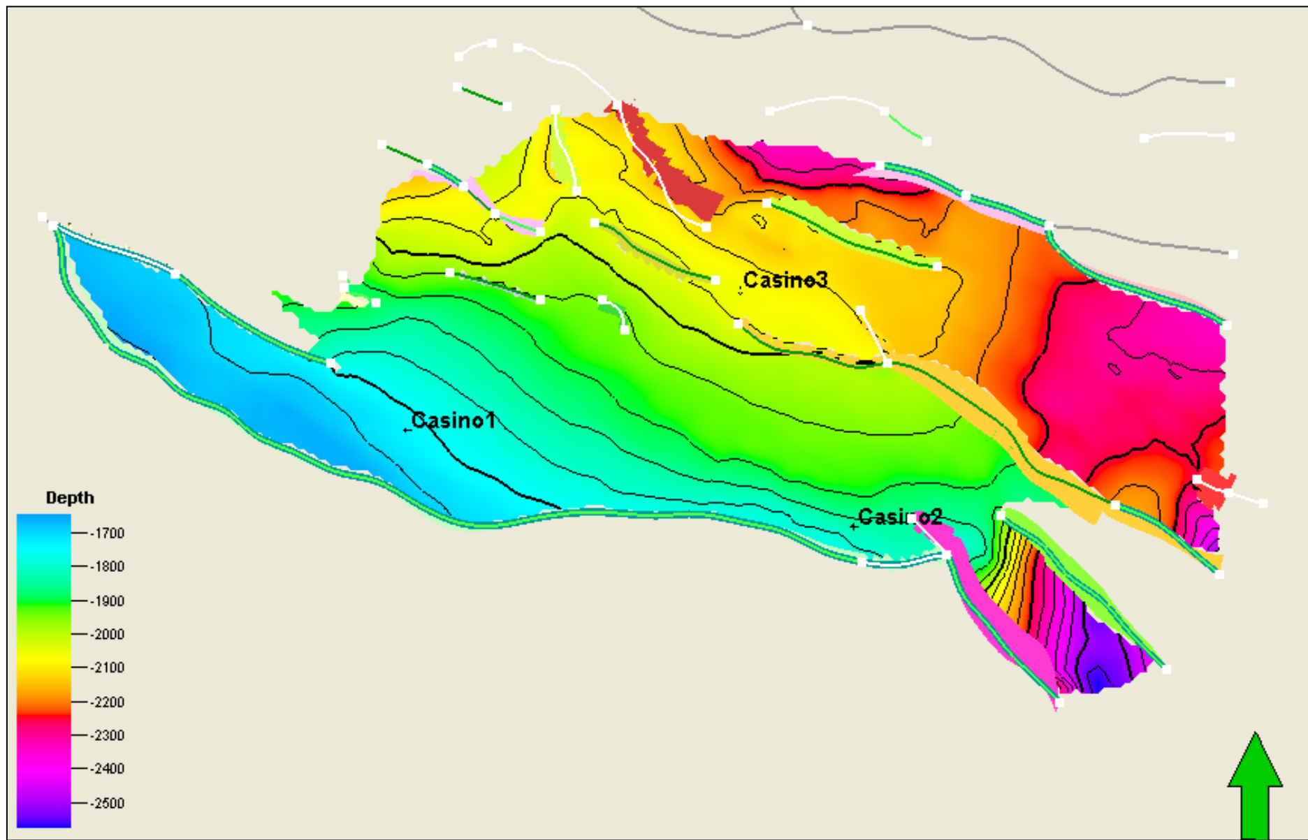
Figure 3.3.3-f: Top Lower Waarre A depth map
