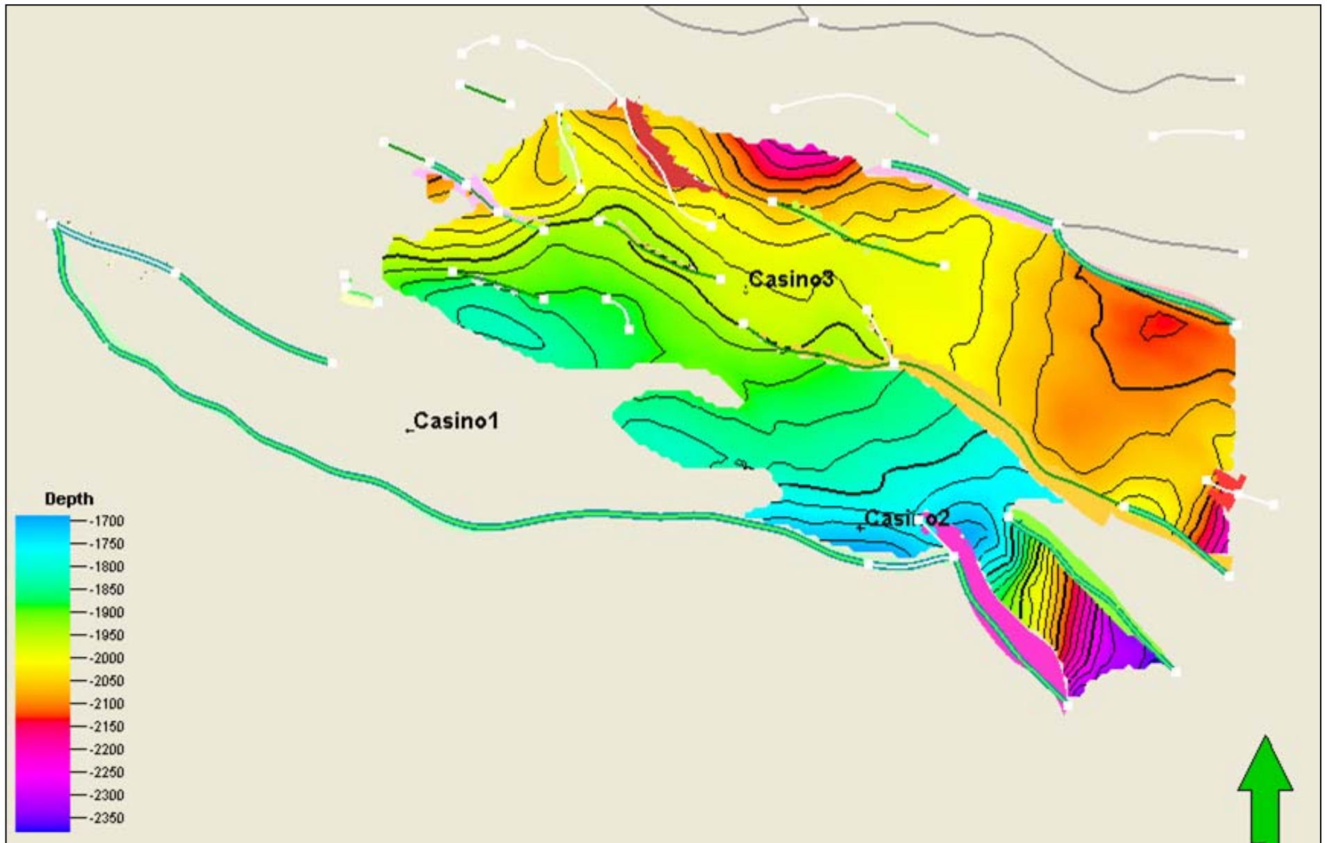
Figure 3.3.3-d: Top Waarre C Main Pay depth map
