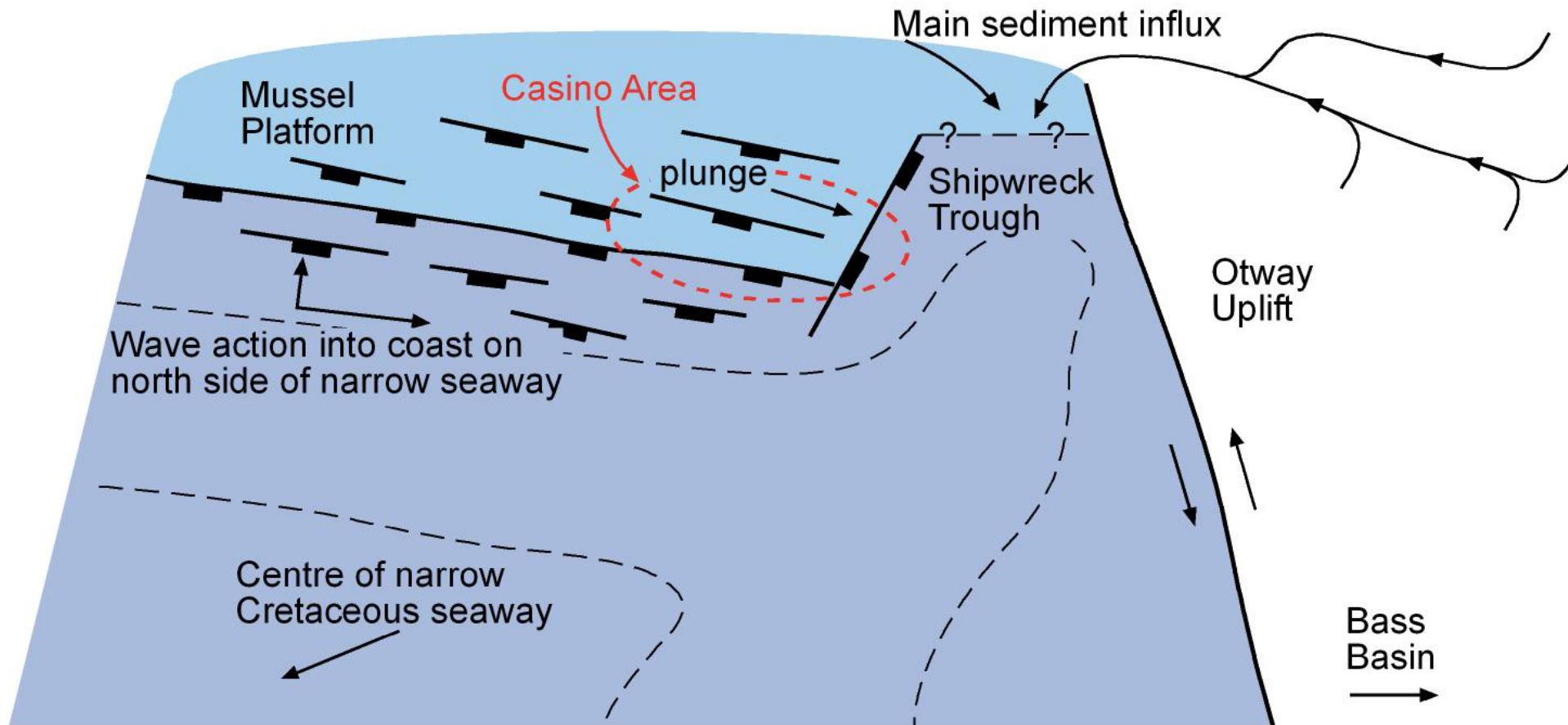
Cartoon of basin geometry at the eastern end of the Cretaceous seaway at its time of deposition of the Waarre Sandstone
