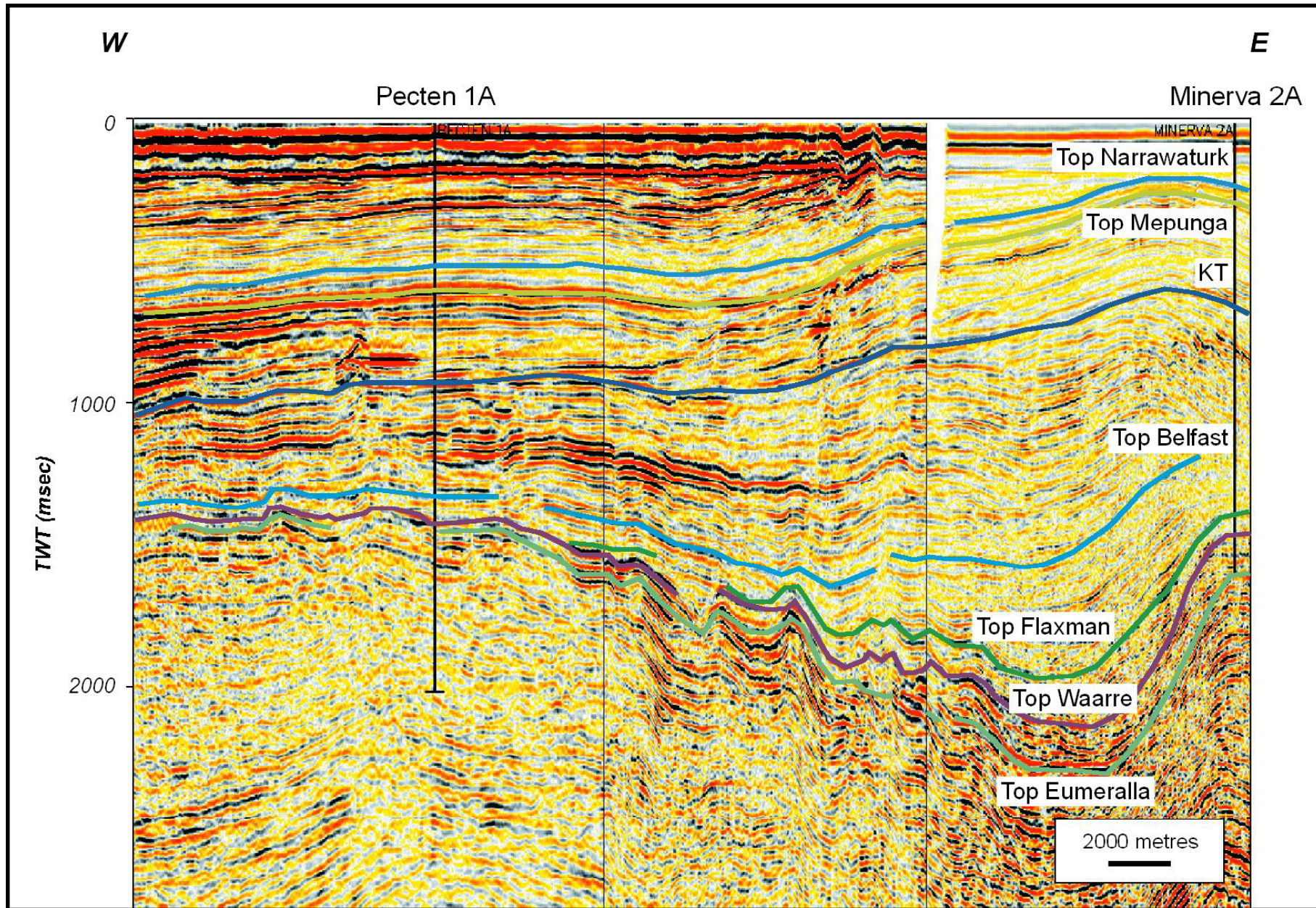
Figure 3.2.1-d: Pecten – Minerva seismic correlation
