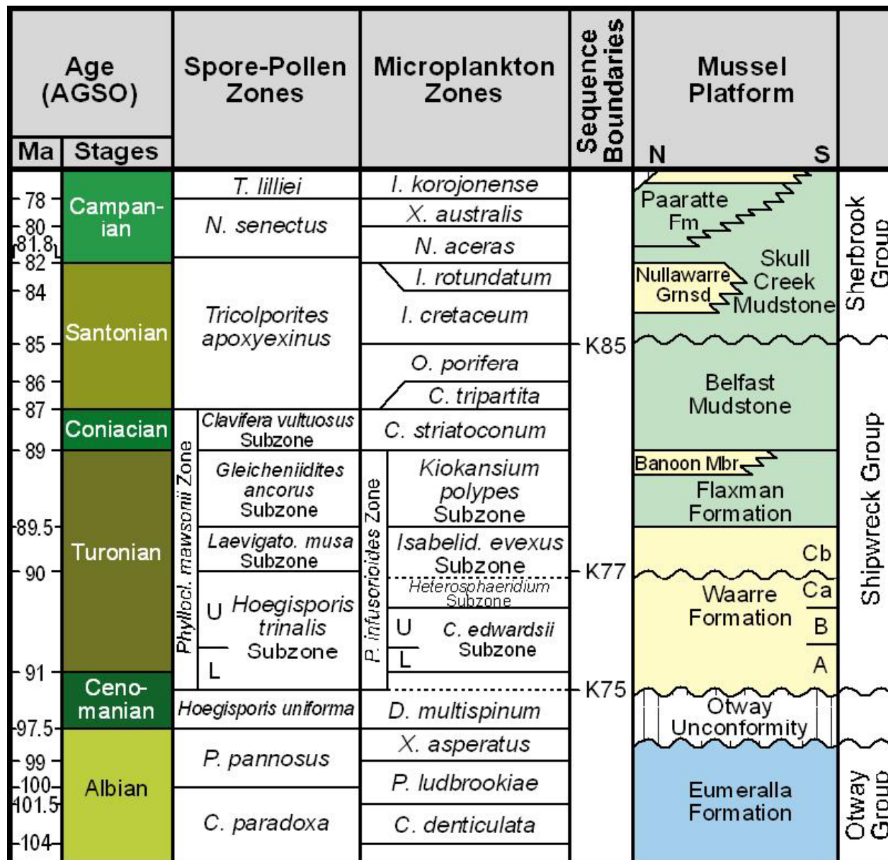
Figure 3.2.1-f: Post Casino-3 stratigraphic chart
