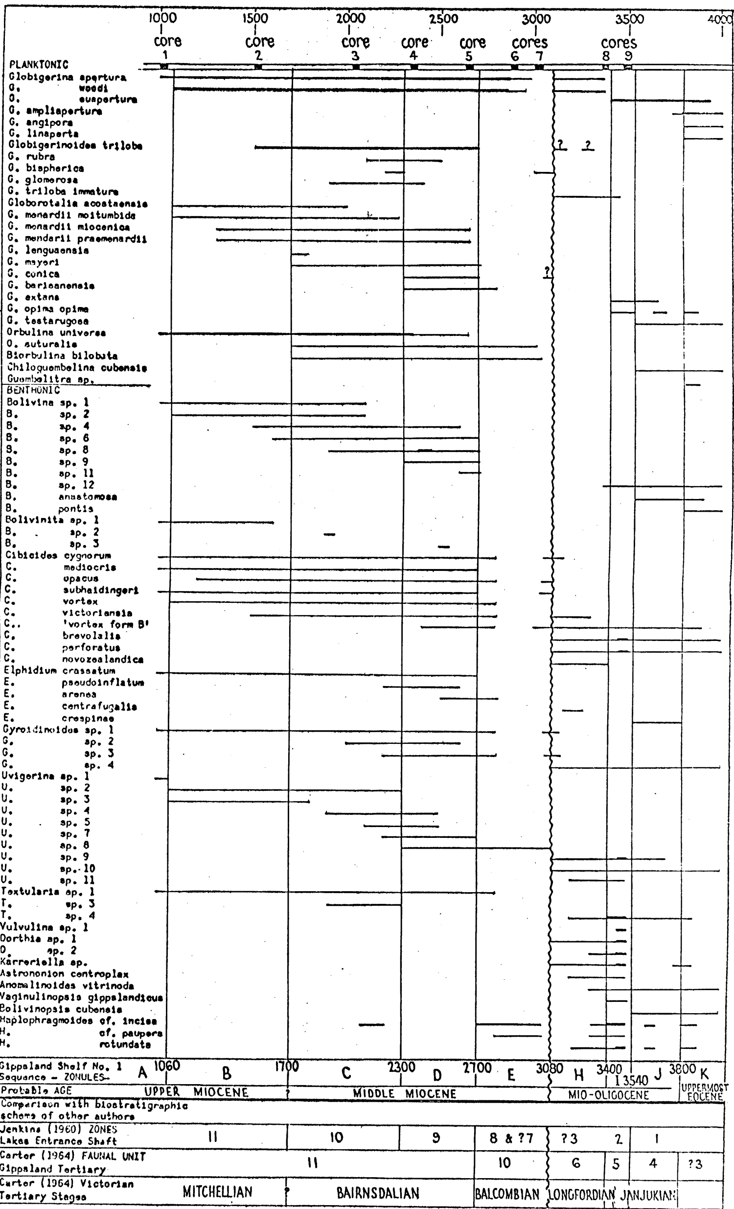
Figure 1 - TERTIARY FORAMINIFERAL DISTRIBUTION
