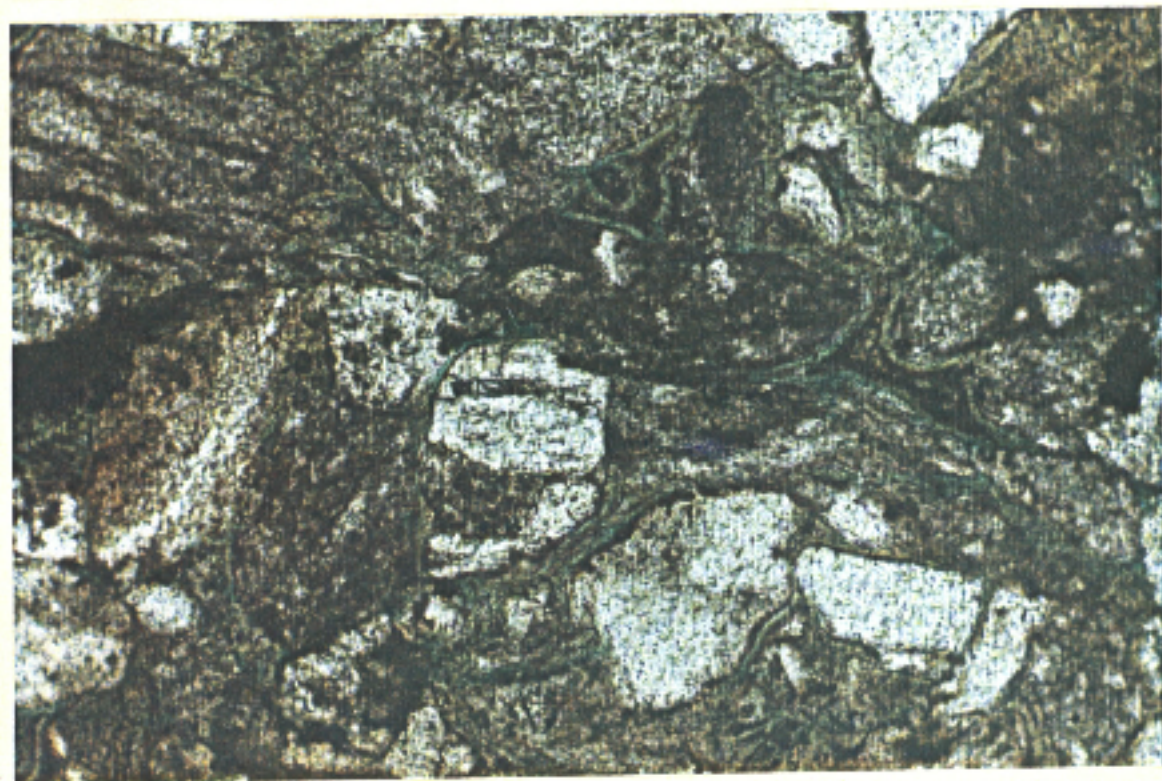
PHOTO 4 1811.0M LITHIC CRYSTAL TUFF SHOWING NARROW CHLORITE RIMS. NIC UNC. FIELD WIDTH 0.7MM
