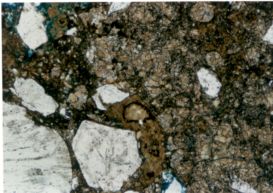
FIGURE 1: Wilson-1, SWC 21. Plane polarised light. Long dimension 2 mm. A field which contains abundant carbonate which possibly shows shadowy outlines of replaced grains. Near bottom centre is a concretion of iron oxide.
