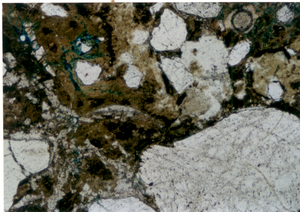
FIGURE 2: Wilson-1, SWC 21. PPL, 2 mm. Field with goethitic matrix and ill-defined concretionary textures. On the left is fine-grained (clear) late carbonate.
