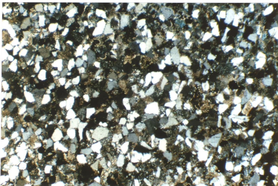
Figure 10: Sample 3: Plain light (upper) and cross-polarised (lower) photomicrograph of fine-grained, well sorted lithic arkose. Long axis of photomicrograph is 3.95mm.
