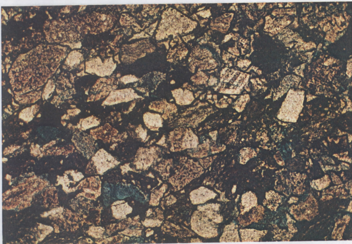
PHOTO 2 P. CAMPBELL 4. CORE 23 7690-7710FT. VOLCANOCLASTIC SHOWING SPORADIC SECONDARY POROSITY.NIC UNC. FIELD WIDTH 1.8MM
