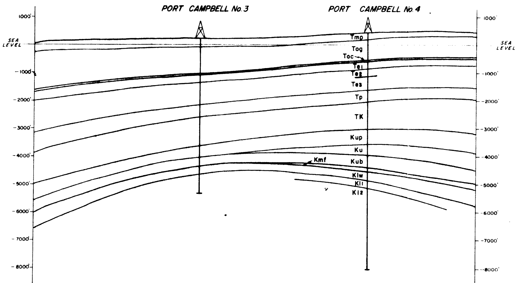
AFTER DRILLING
