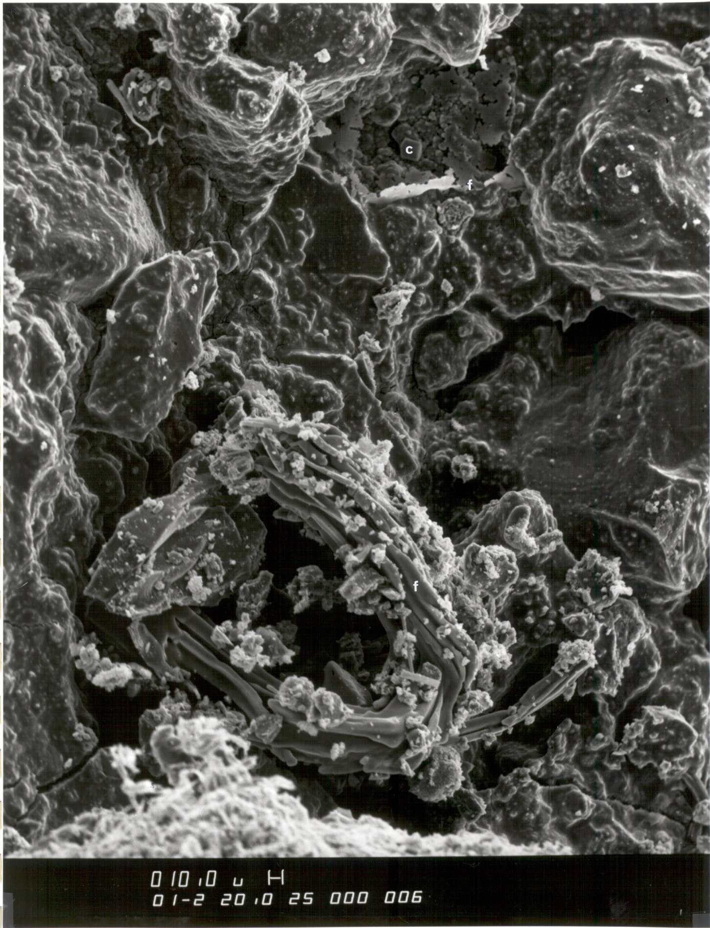
PLATE 8: 2044.5 m The partially dissolved grains in this field (f) were probably feldspars. These grains were likely to have been dissolved earlier in the diagenetic history when the sandstone was more permeable.
