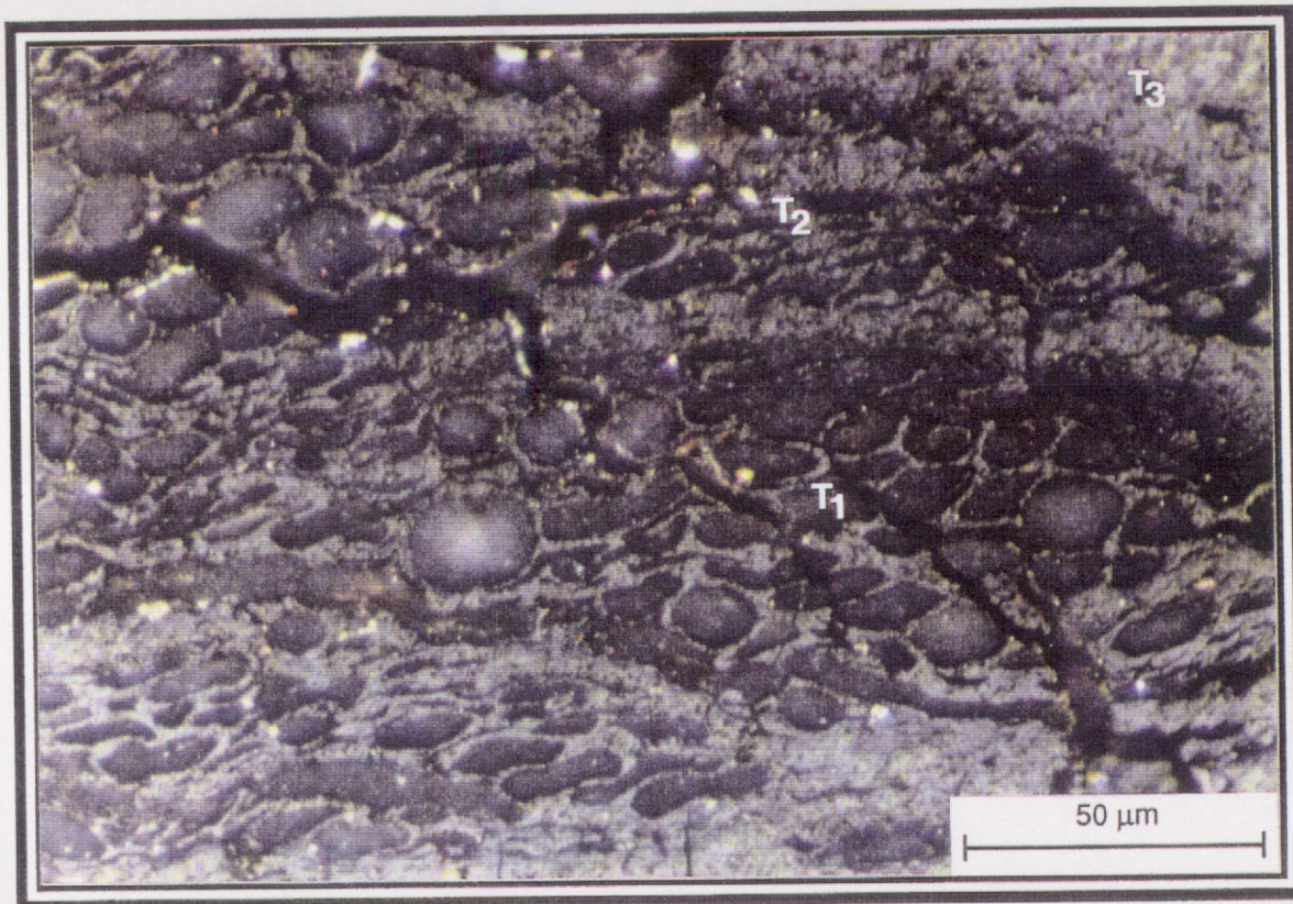
PLATE 5a: Photomicrograph showing coal, microlithotype vitrite. Texto-ulminite (T1), eu-ulminite (T2) and telocollinite (T3). [Sample A-923.186, 213.6m, oil immersion, reflected light, X50].
