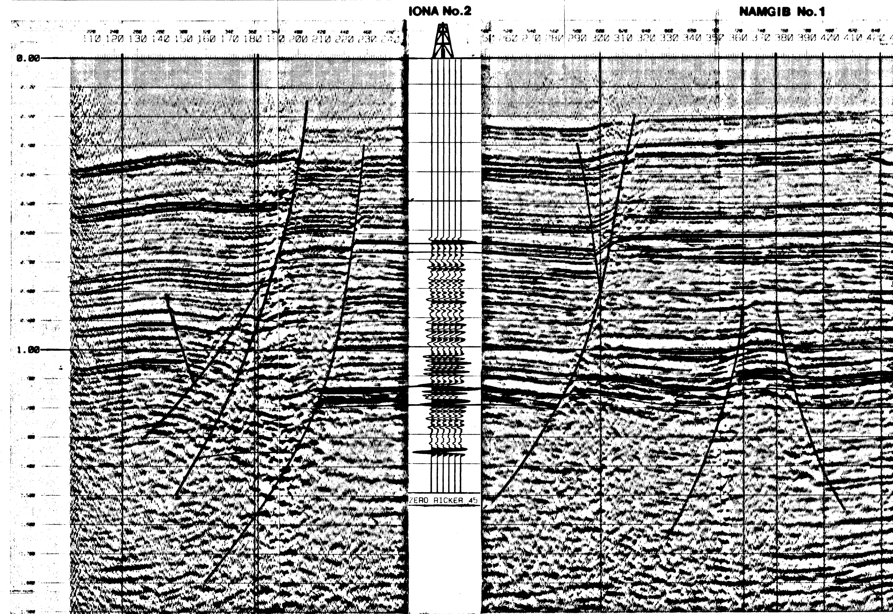
SEISMIC LINE : IONA93-01
