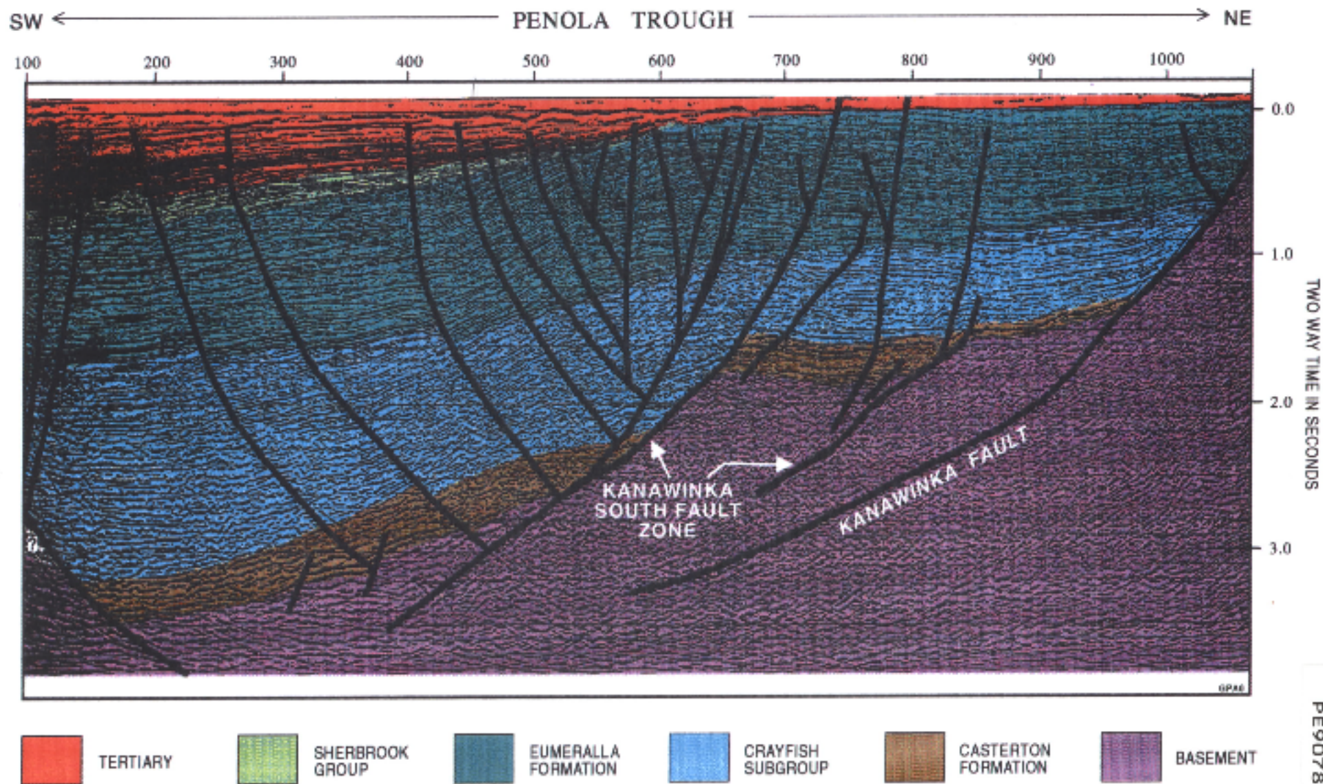
FIGURE 4.4: BEACH PETROLEUM SEISMIC LINE HF88-14 SHOWING THE NORTHERN PART OF THE PENOLA TROUGH (Seismic line courtesy of SANTOS)
