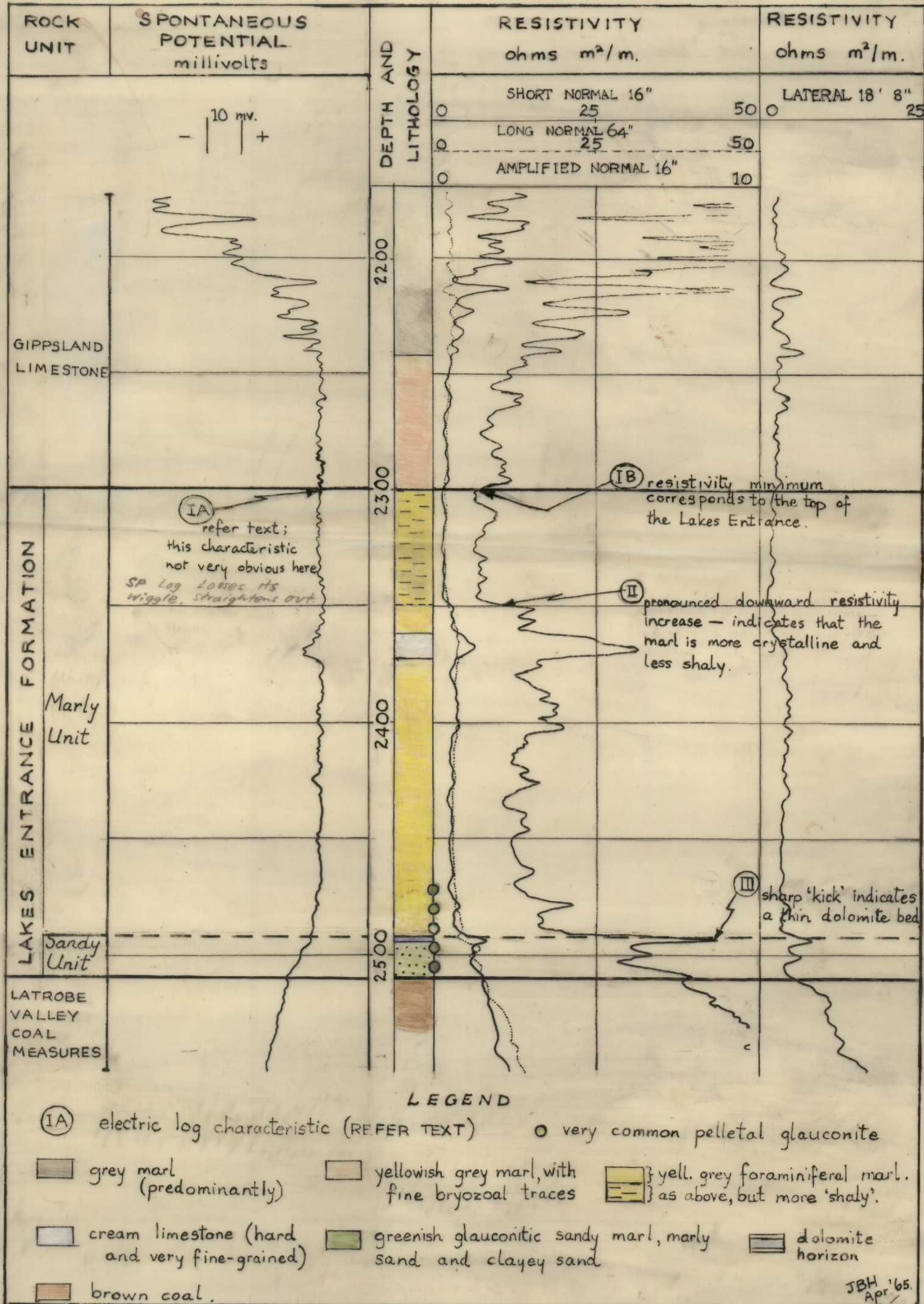
FIG. 5. ELECTRIC LOG CHARACTERISTICS OF THE LAKES ENTRANCE FORMATION [EXAMPLE: WOODSIDE No. 2 WELL].
