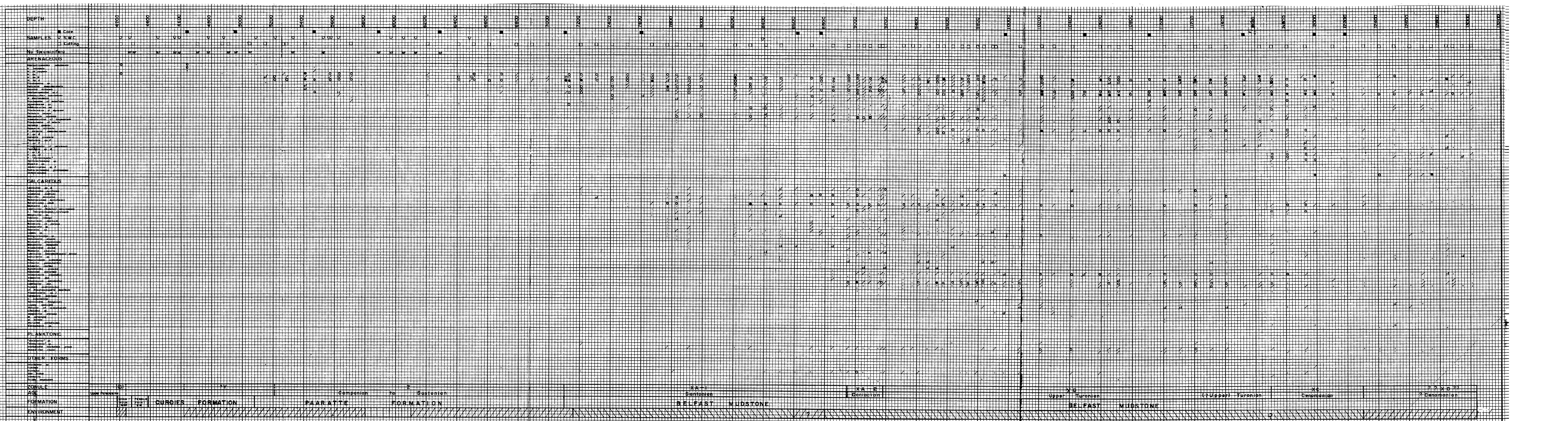
DISTRIBUTION OF SELECTED FORAMINIFERA VOLUTA-1 (EXCLUDING UPPER TERTIARY) AND DEPOSITIONAL ENVIRONMENT Scale 1" to 200'
