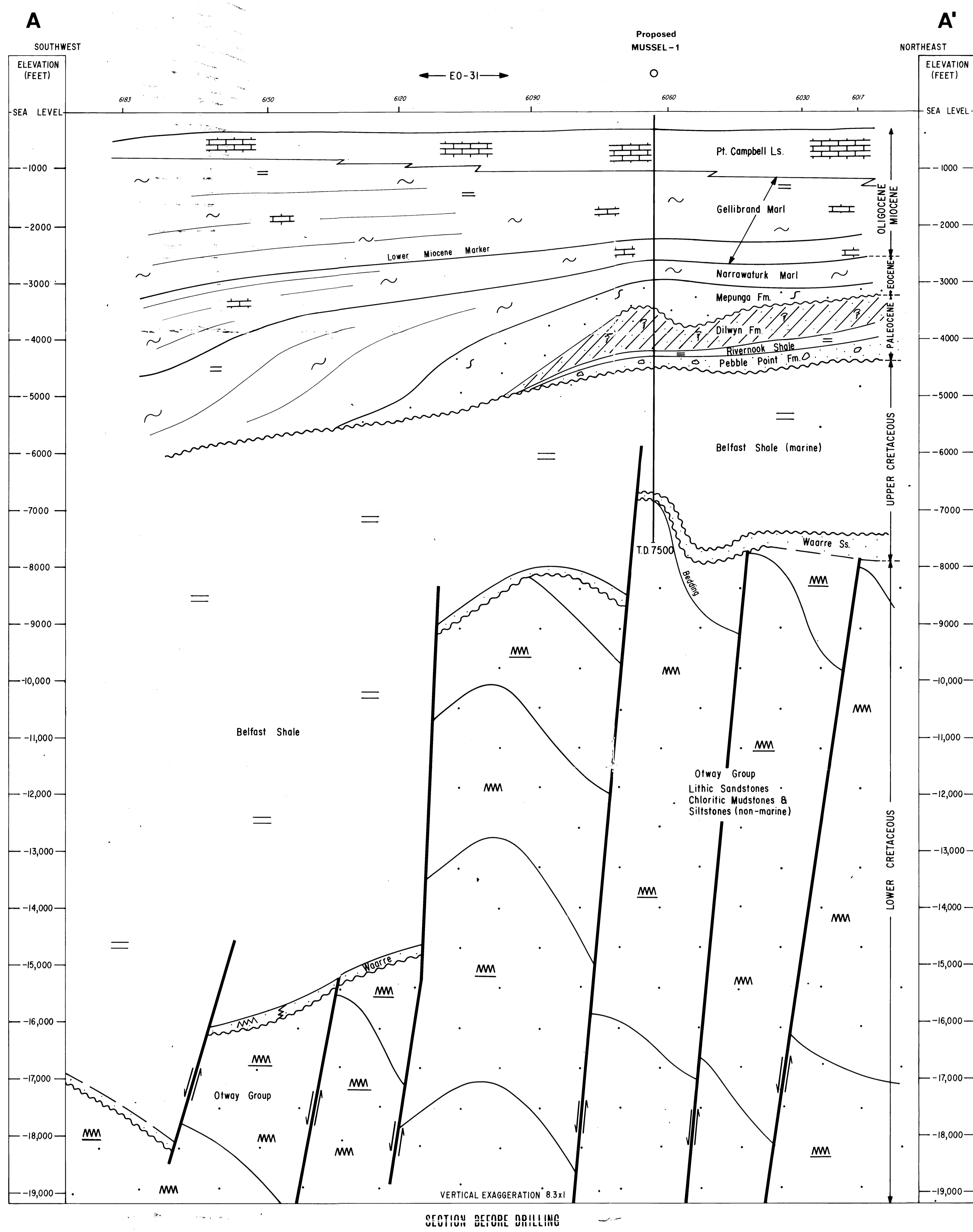
SECTION BEFORE DRILLING
