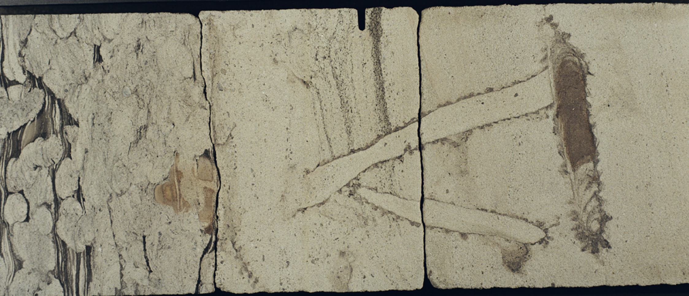
SANTOS CASINO#2. CORE 1 1766.6 to 1766.9m
