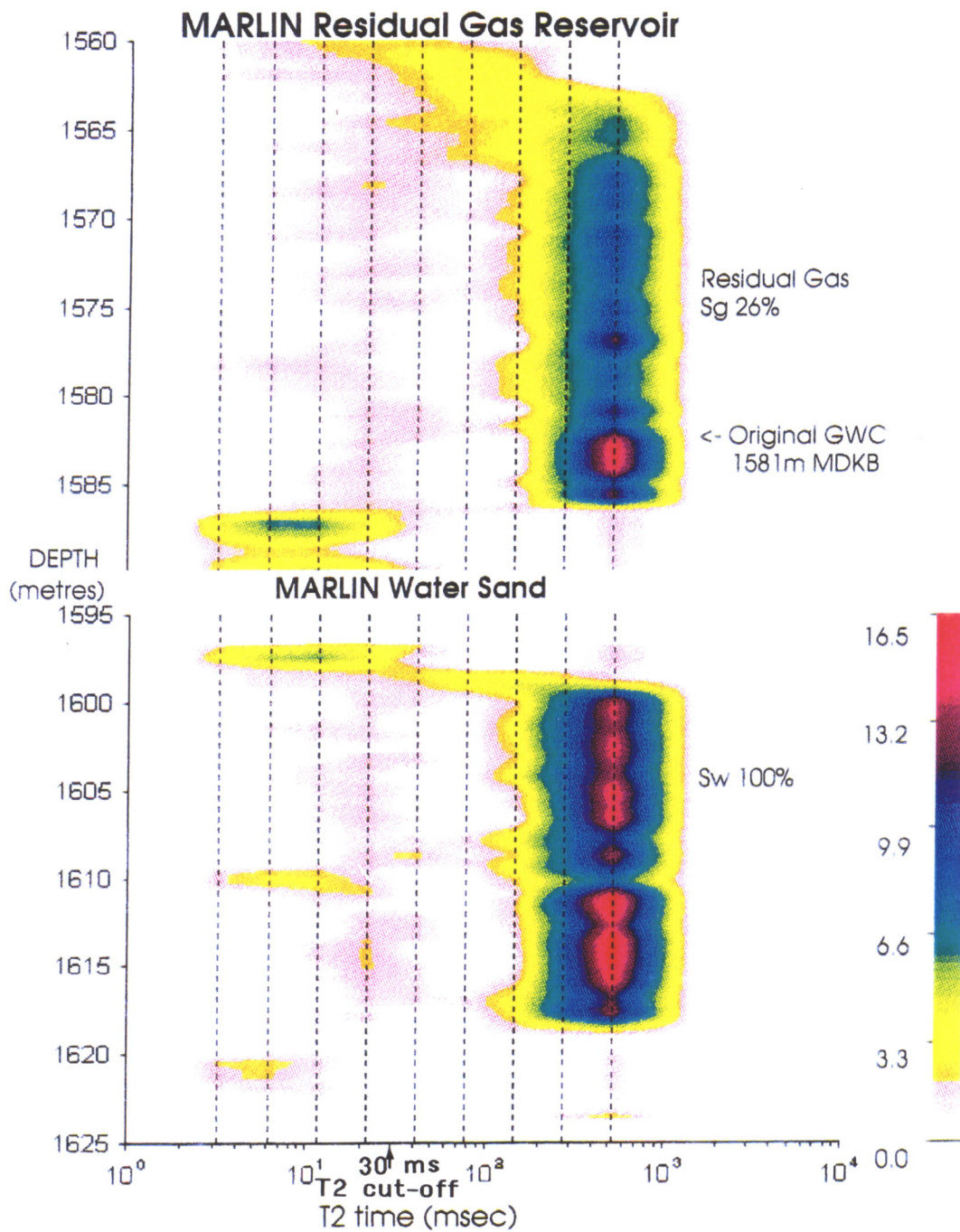
Figure 3 MRIL T2 distribution in residual gas column shows decreased signal amplitude above Marlin original gas-water contact, 1581 metres. Strong uni-modal signal amplitude throughout high porosity sand may be caused by bulk fluid T2 relaxation.
