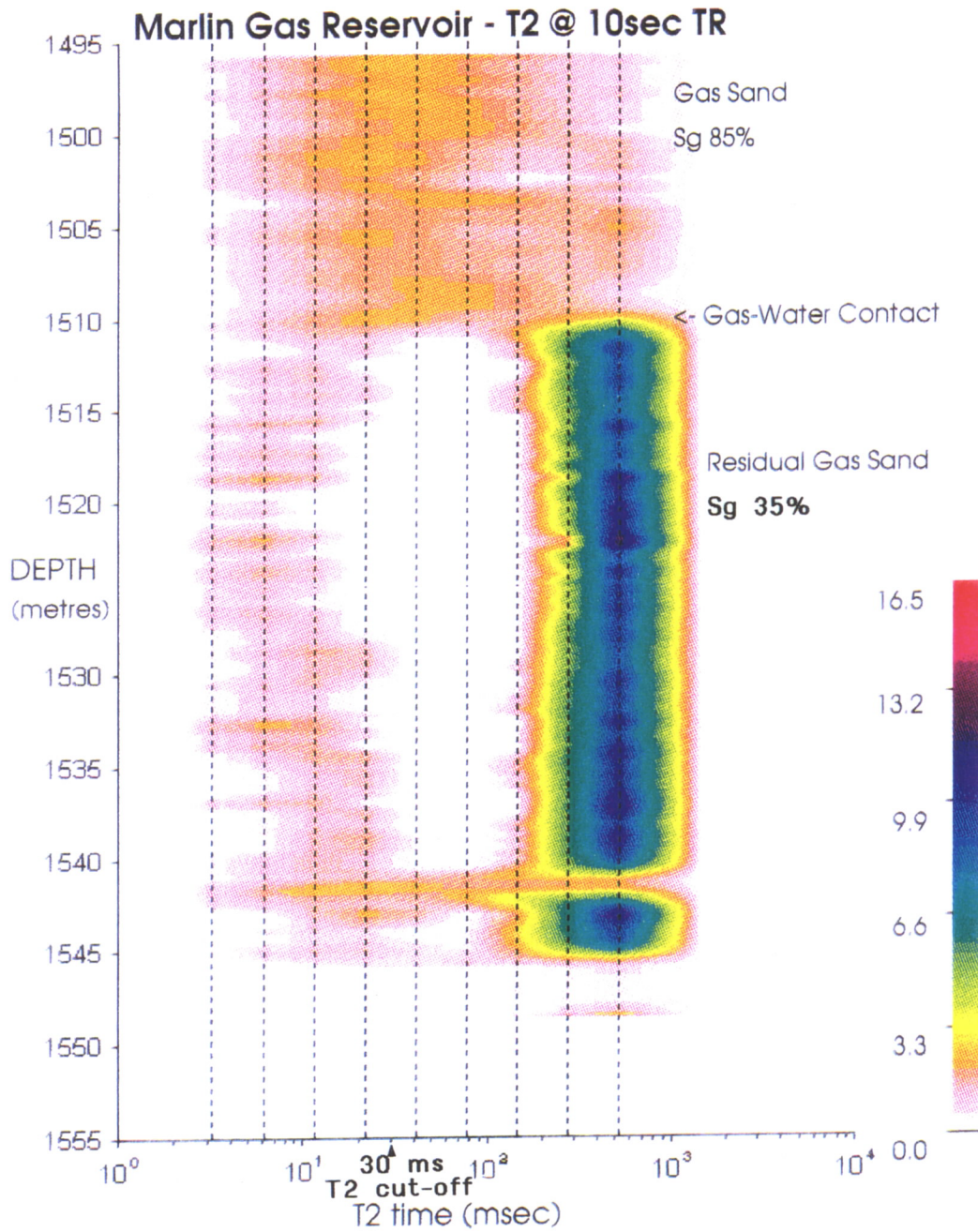
Figure 2 MRIL T2 distribution shows abrupt loss of signal at present day gas-water contact, 1510 metres. T2 diffusion of gas is 18 msec, which places observed signal in BVI window (<30 msec).
