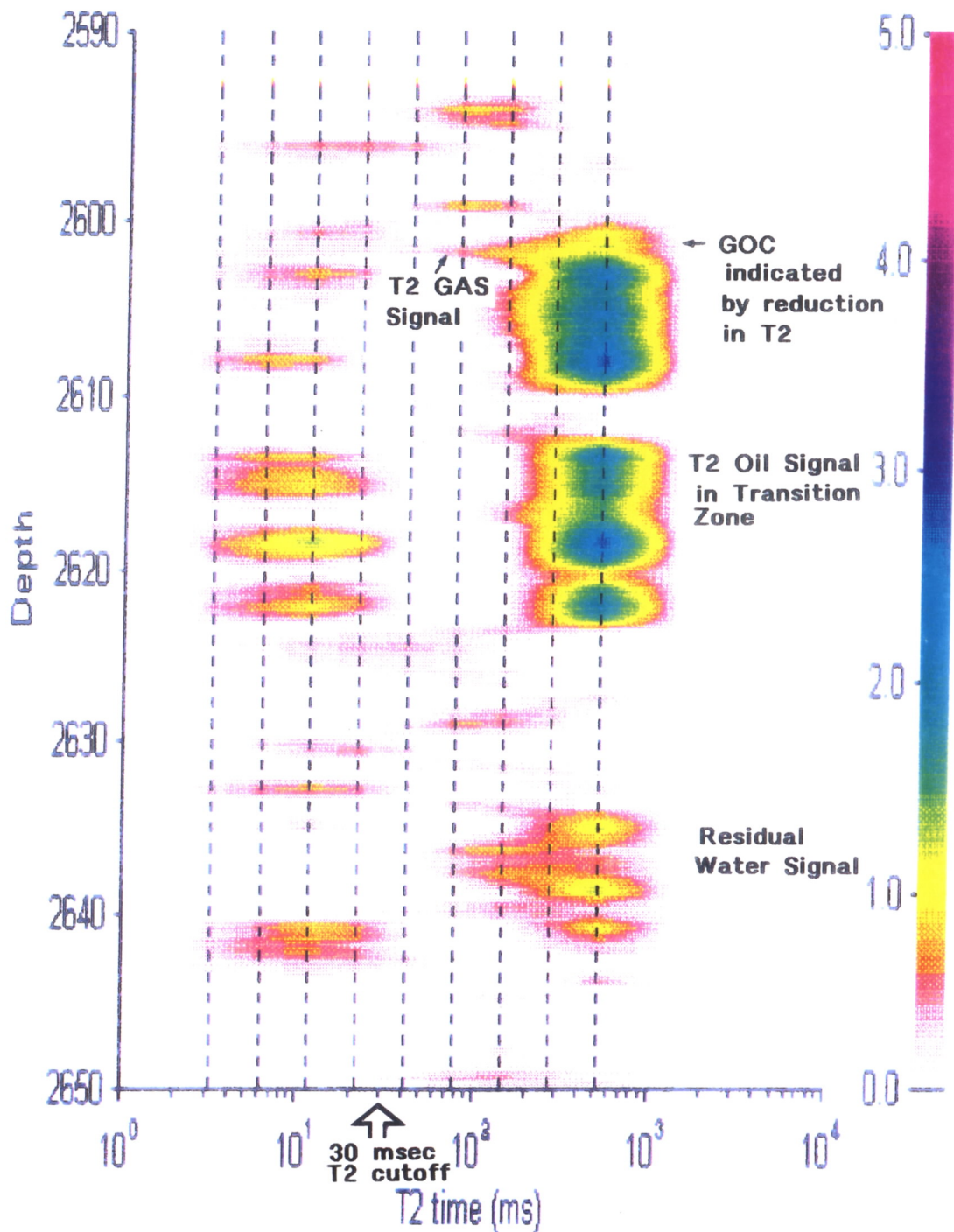
Figure 3 Turrum 5 MRIL T2 differential spectrum (Method A) removes most of the water signal and shows a strong oil signal at 500 msec. The L500 GOC is identified by reduction in T2 at 2602 metres. A small residual water signal remains in the water leg below 2628 metres. Note the absence of the free water signal in the transition zone between 2612 to 2623 metres.
