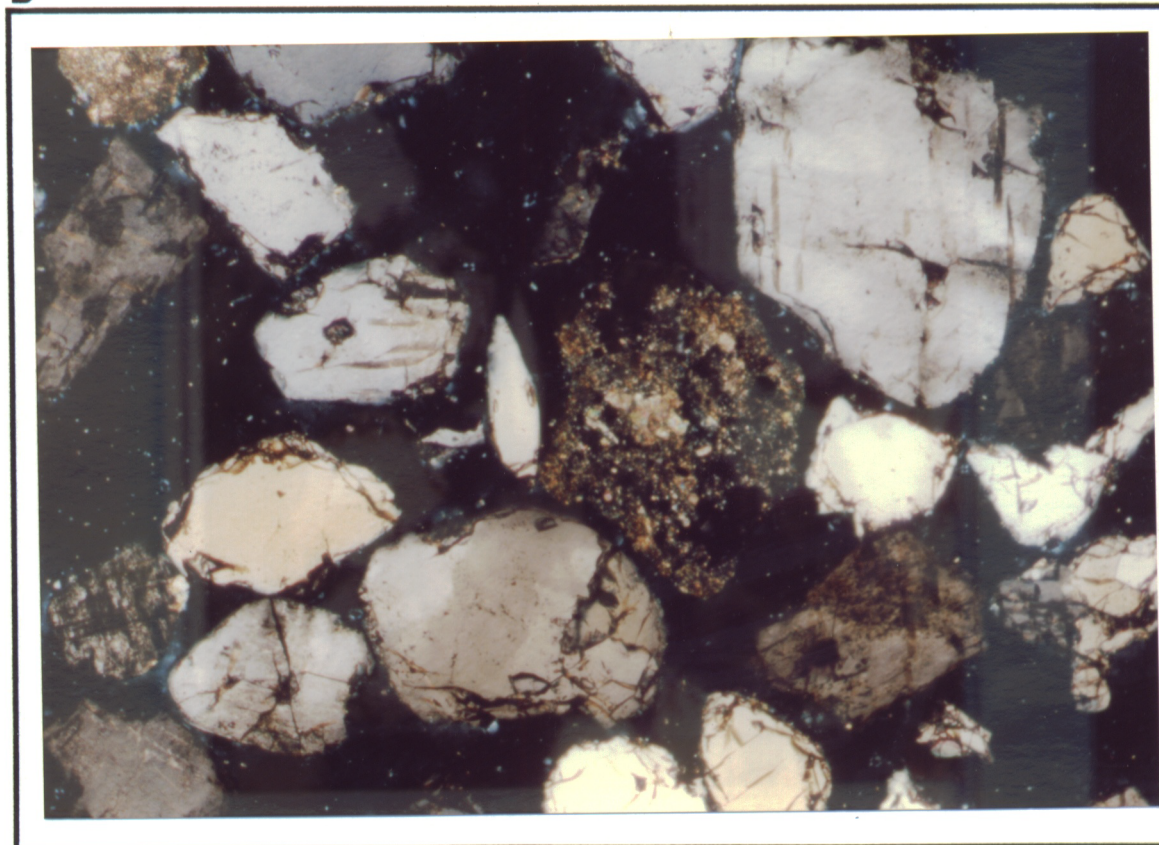
Figure 6: GC333-6, Devilfish-1, cuttings. Latrobe Group quartz sandstone. Free granitic quartz dominant, some sericitized K-feldspar (note the blue dye does not indicate 1° porosity in this cuttings sample). Calcite cemented foraminifera present. Diagenetic kaolonite very rare.
