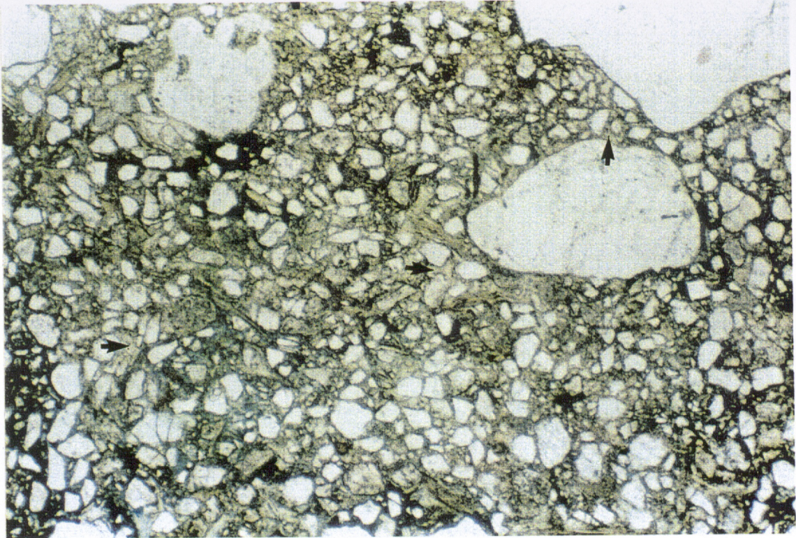
Figure 10a. Thin section photomicrograph of bimodal, micaceous quartzarenite with pore spaces occluded by chlorite (arrows). Mudskipper #1, depth 1598.5m. Plane light. Field of view 2.72mm.
