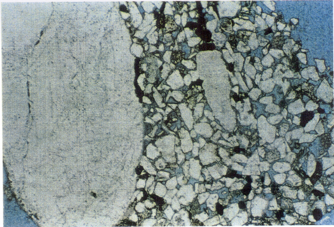
Figure 4. Thin section photomicrograph of bimodal subarkose with intergranular porosity. Mudskipper #1, depth 1607.5m. Plane light. Field of view 2.40mm.
