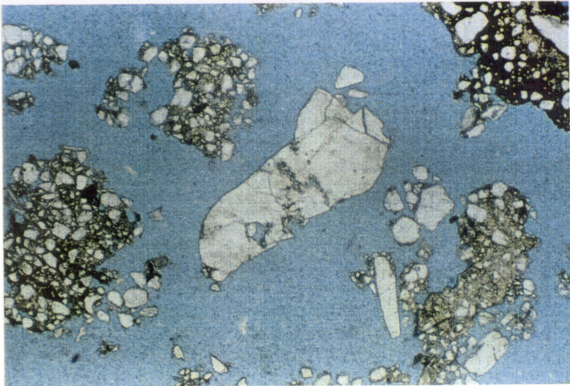
Figure 5. Thin section photomicrograph of secondary dissolution in feldspar grain. Mudskipper #1, depth 1607.5m. Plane light. Field of view 2.72mm.
