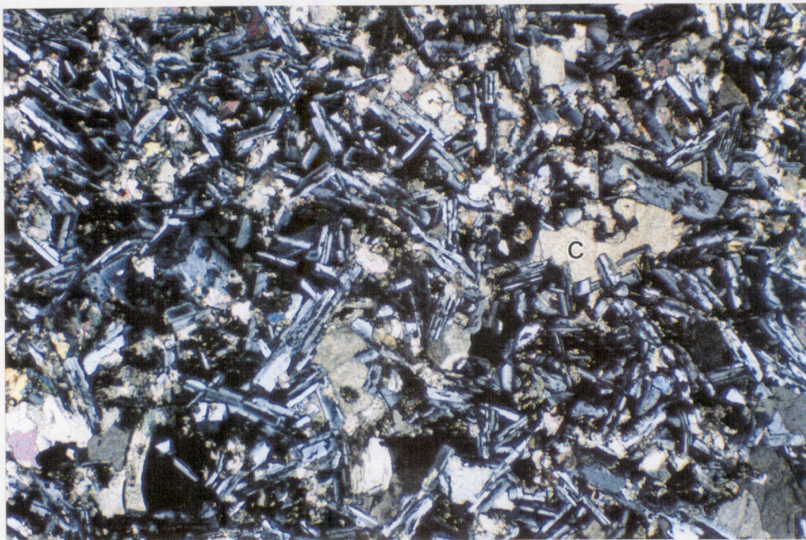
Figure 3: Sample 9 (2104.5 m): Plain (upper) and cross polarised (lower) photomicrographs of plagioclase-rich basalt. This comprises plagioclase lathes (P) and calcite (C) possibly replacing pyroxene. Long axes of photomicrographs are equal to 2.72 mm.
