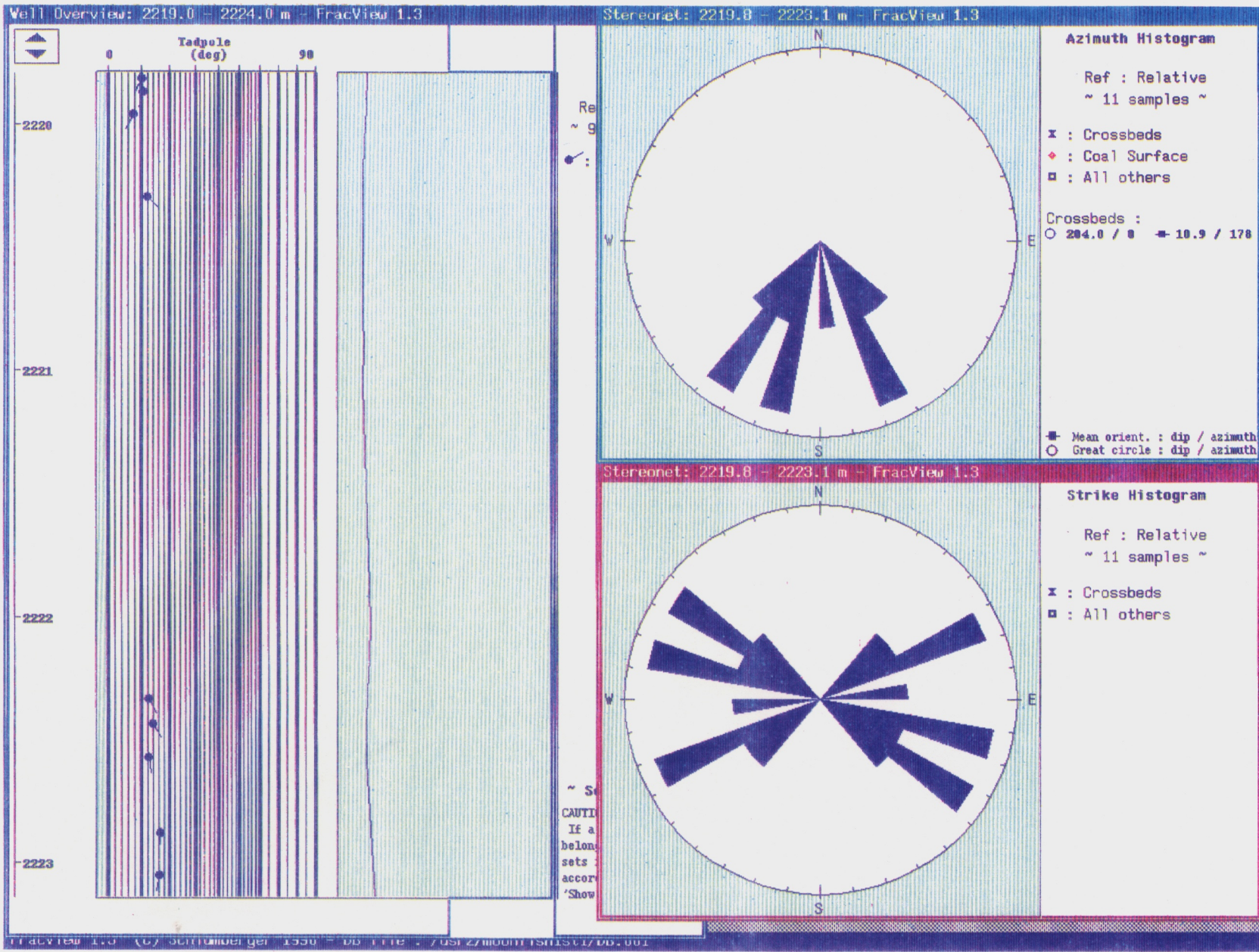
FIGURE 16 Crossbeds SDR Dip Azimuth 178° Interval 2219m to 2224m.
