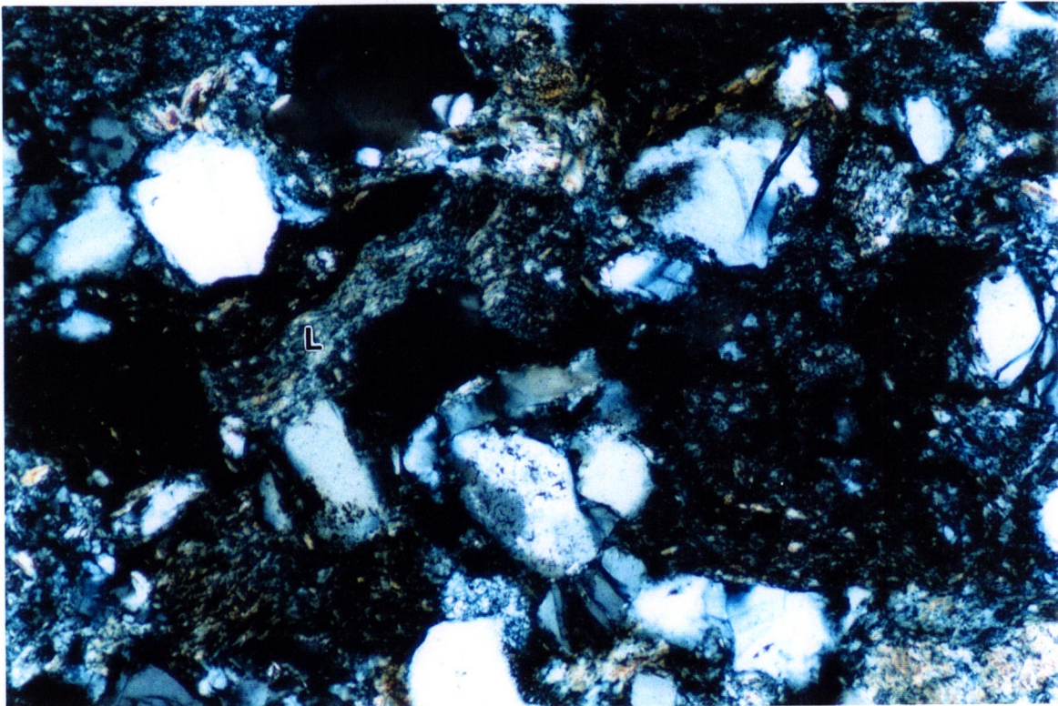
Figure 4: Sample 23 (1899.5 m): Plain (upper) and cross-polarised (lower) photomicrographs of litharenite. This sample displays moderate impact damage. Nevertheless, a compacted micaceous lithic grain (L) is evident and shows long grain contacts with surrounding grains. Destruction of pore throats at long grain contacts has significantly reduced permeability. Long axis of photomicrograph is equal to 0.88 mm.
