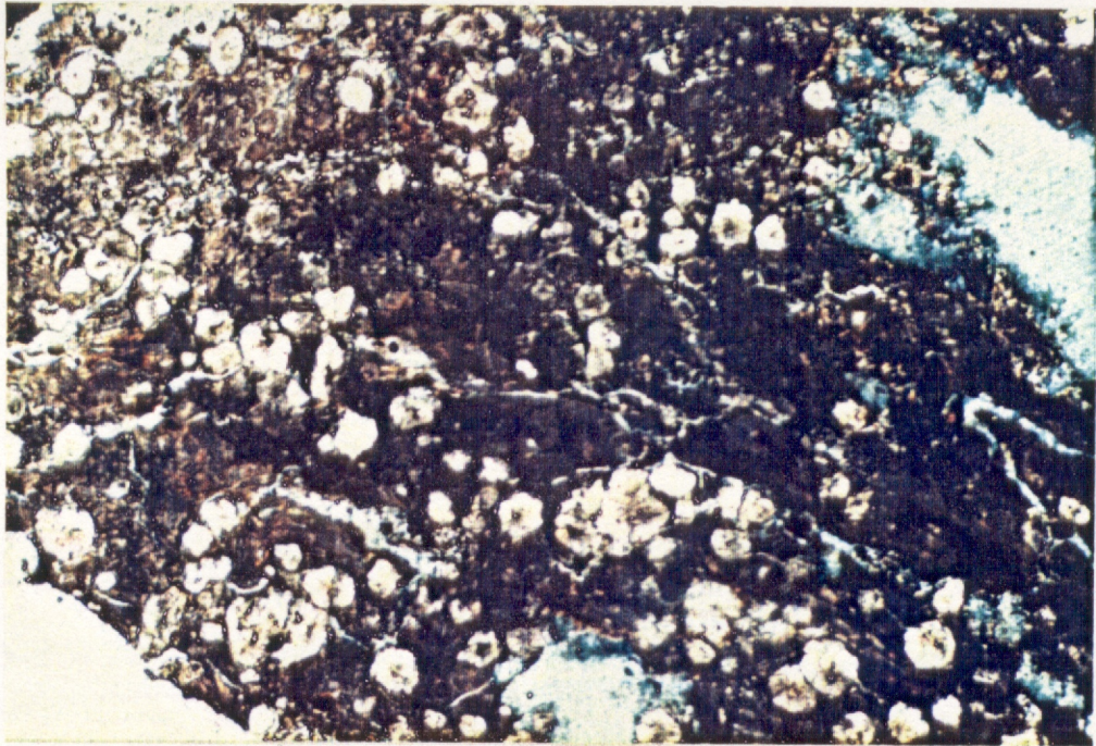
PLATE 3: SAMPLE SWC9 - OOLITES OF CARBONATE (white) IN VARIOUSLY COLOURED CLAYS FROM ALTERED FELSIC PYROCLASTS. (x14 magnification)
