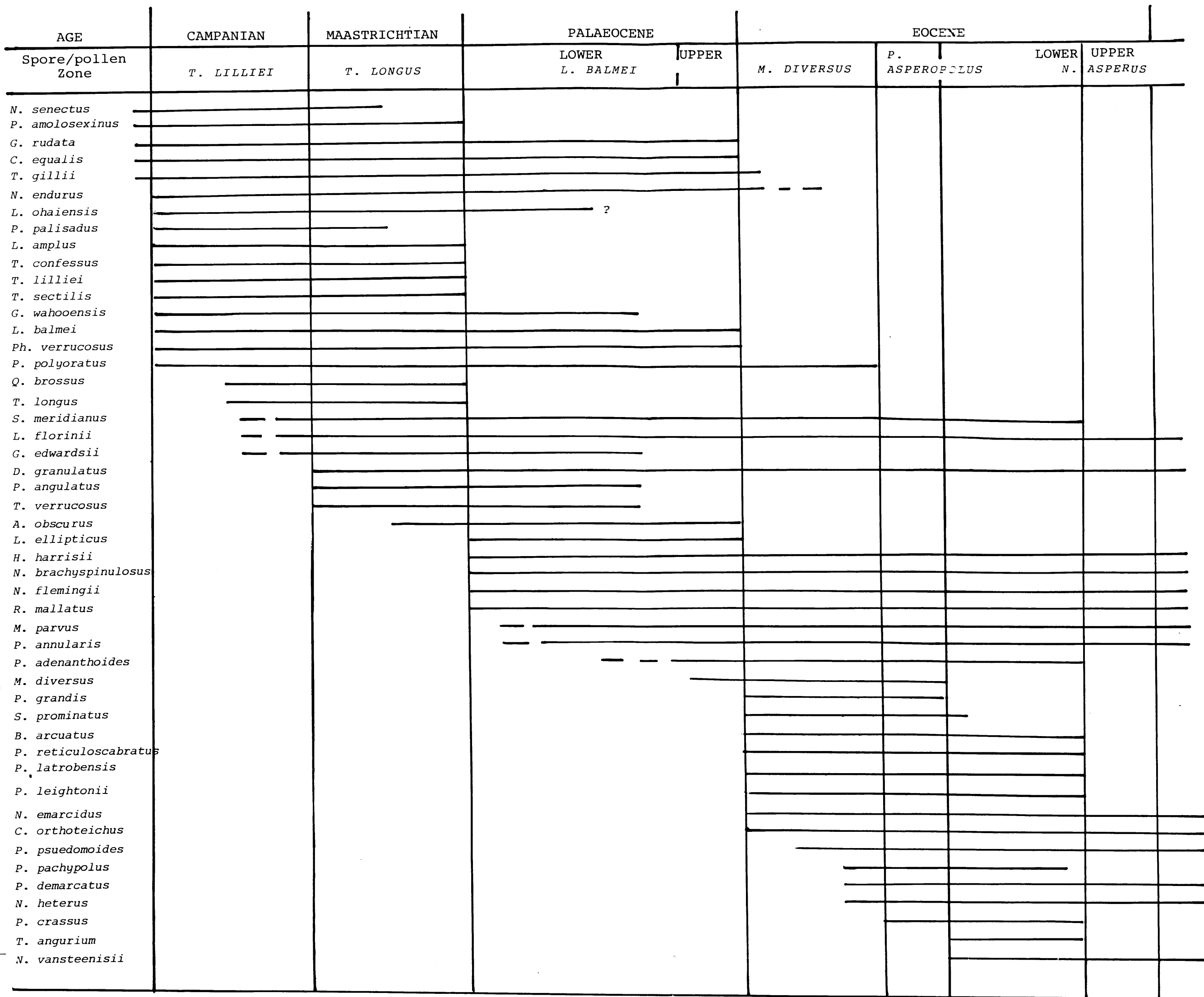
FIGURE 1: HELIOS # 1 SPORE POLLEN RANGE CHART COMPILED FROM STOVER & PARTRIDGE, 1973 and PARTRIDGE, 1976.
