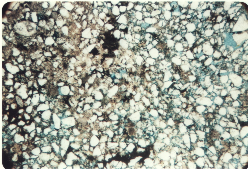
Figure 11. Latrobe Group 1325m. Typical clean, quartz sand (stone) with minor pyrite and feldspar. Blue is porosity. Field of view ca 4.4mm. Plane polarized light.
