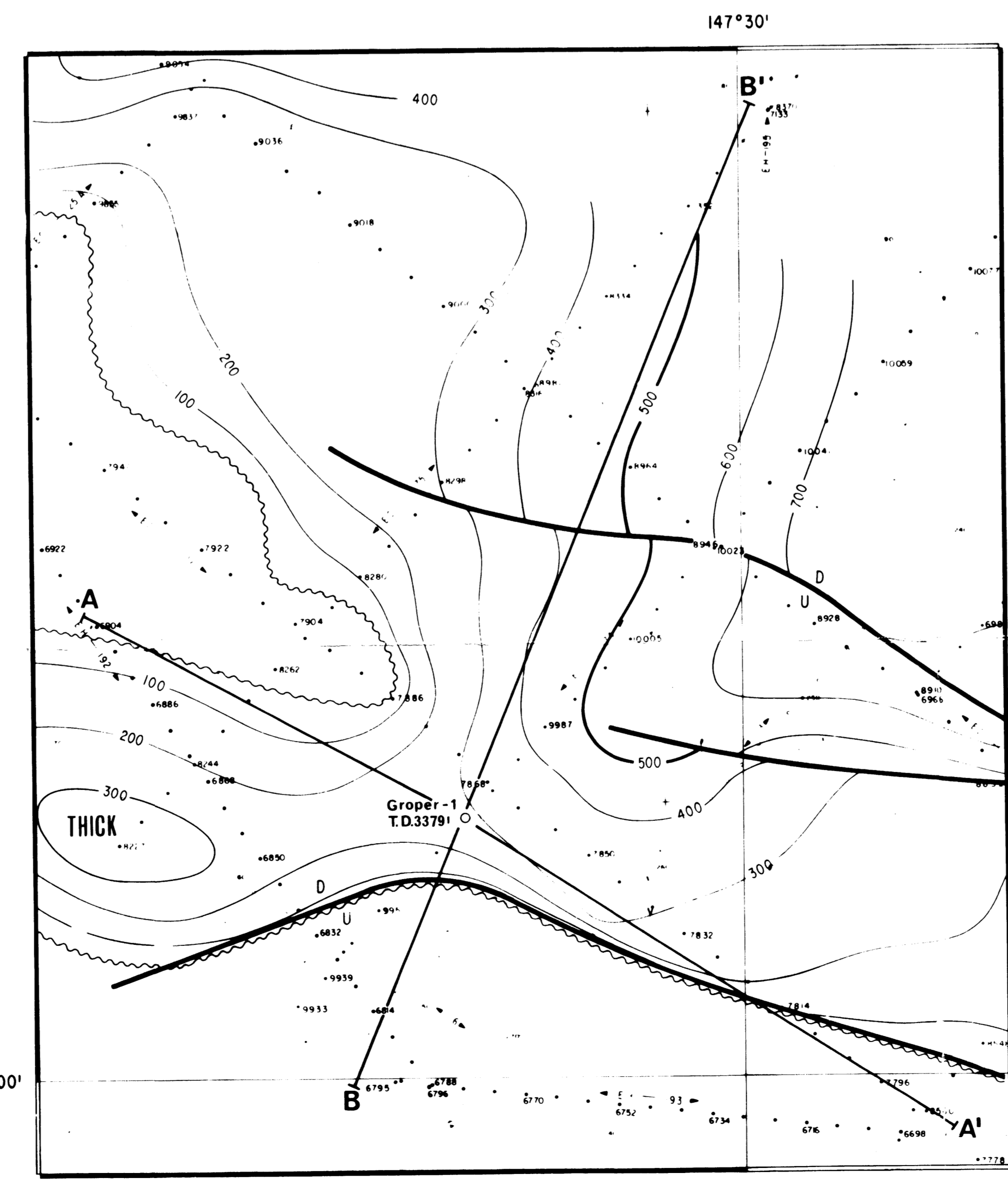
ISOPACH MAP - LATROBE DELTA COMPLEX
