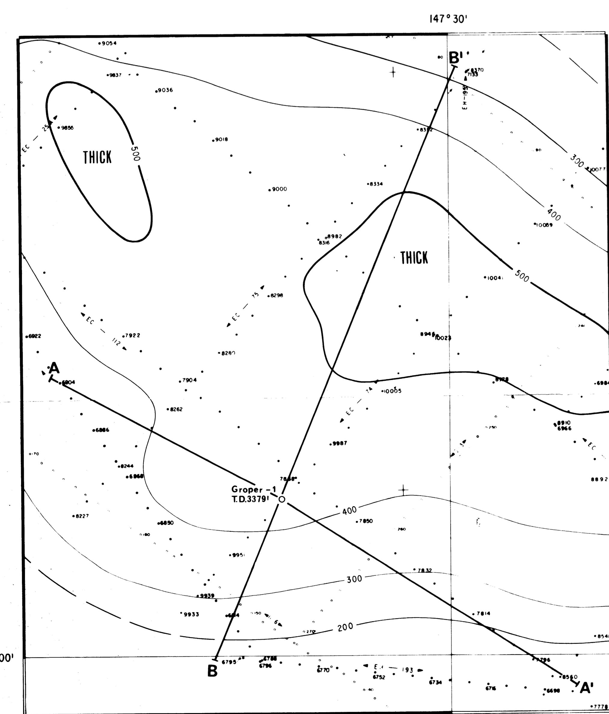
ISOPACH MAP - LAKES ENTRANCE FORMATION
