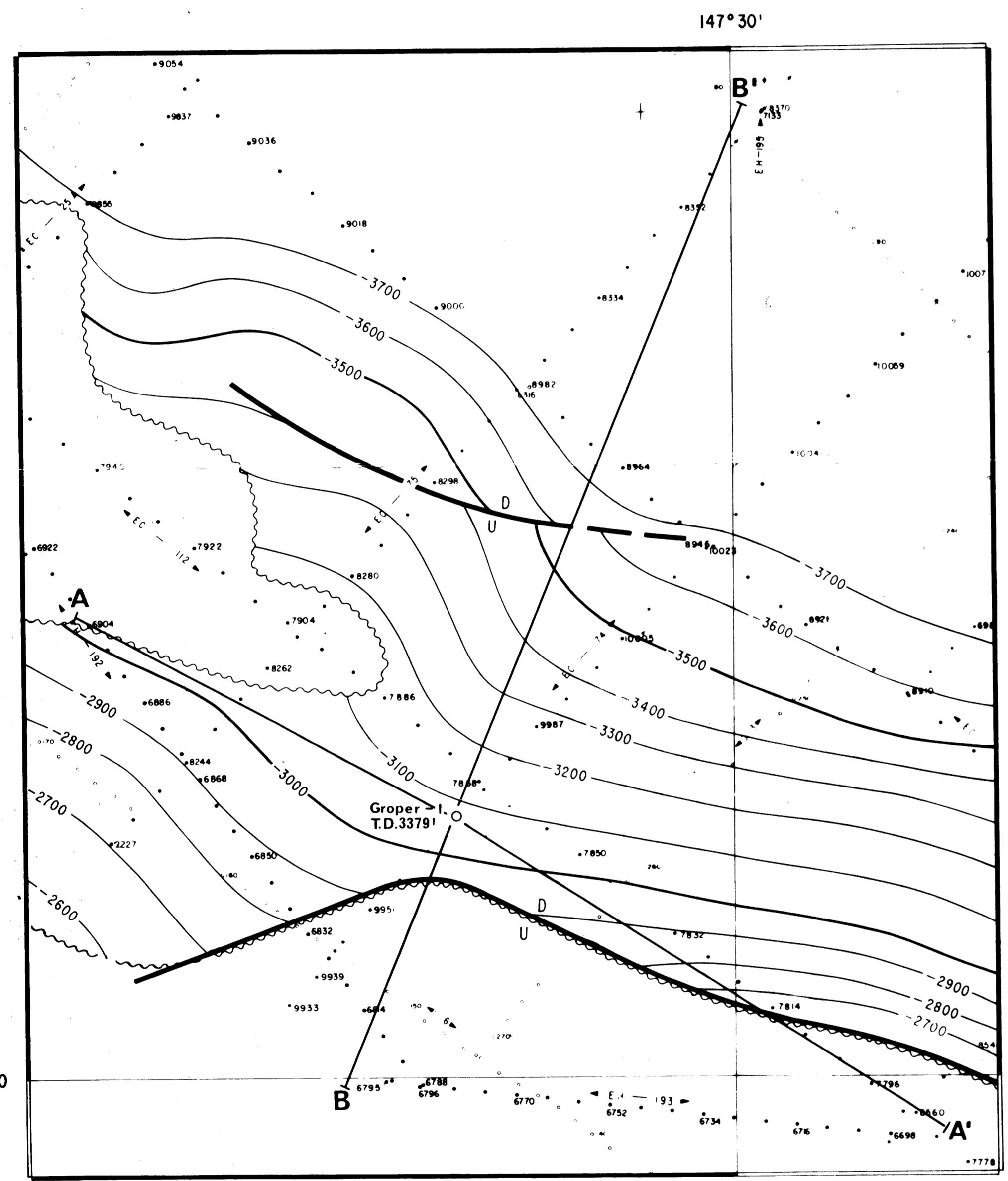
STRUCTURE MAP - LATROBE DELTA, TOPOGRAPHIC SURFACE
