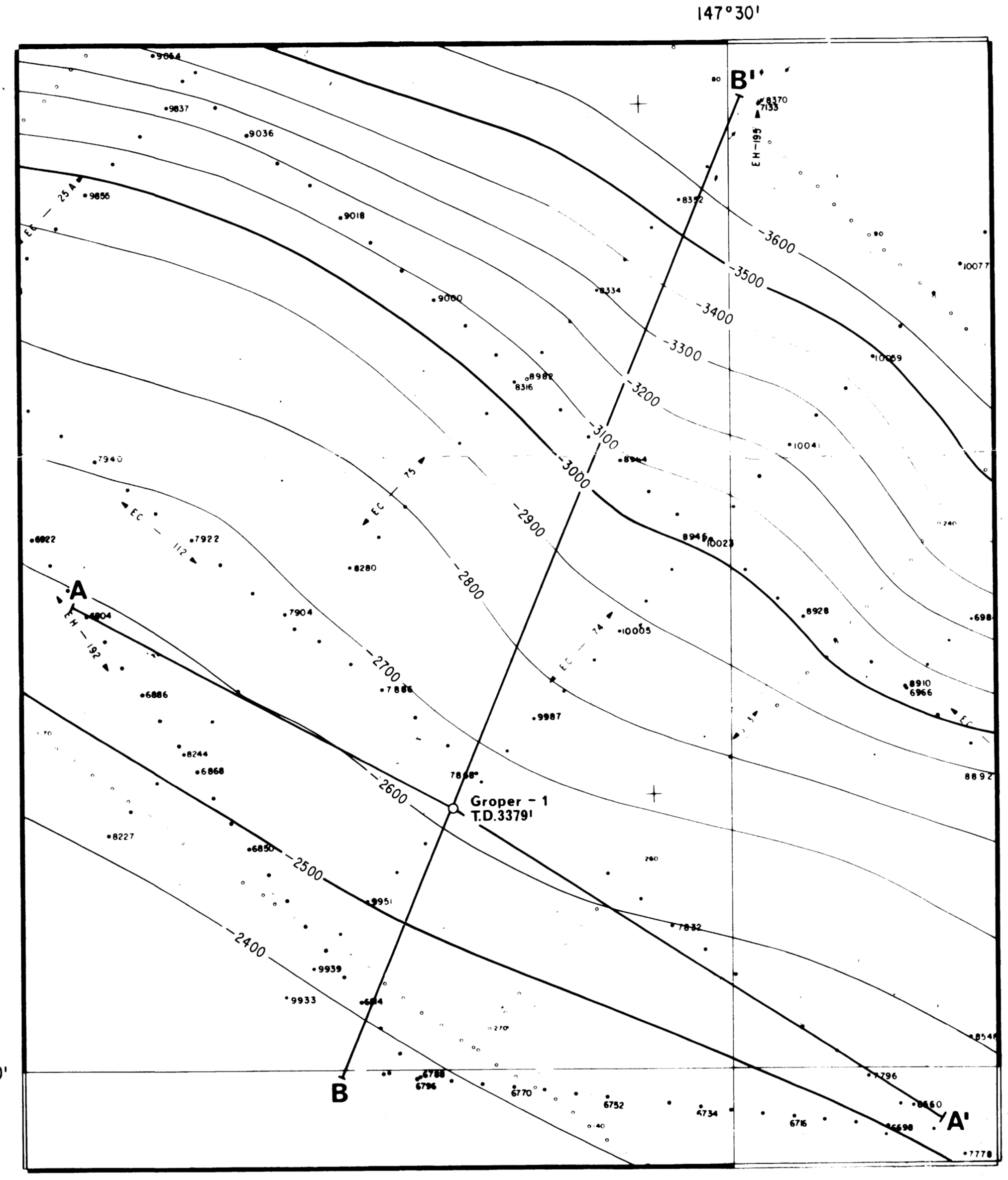
STRUCTURE MAP - LAKES ENTRANCE FORMATION
