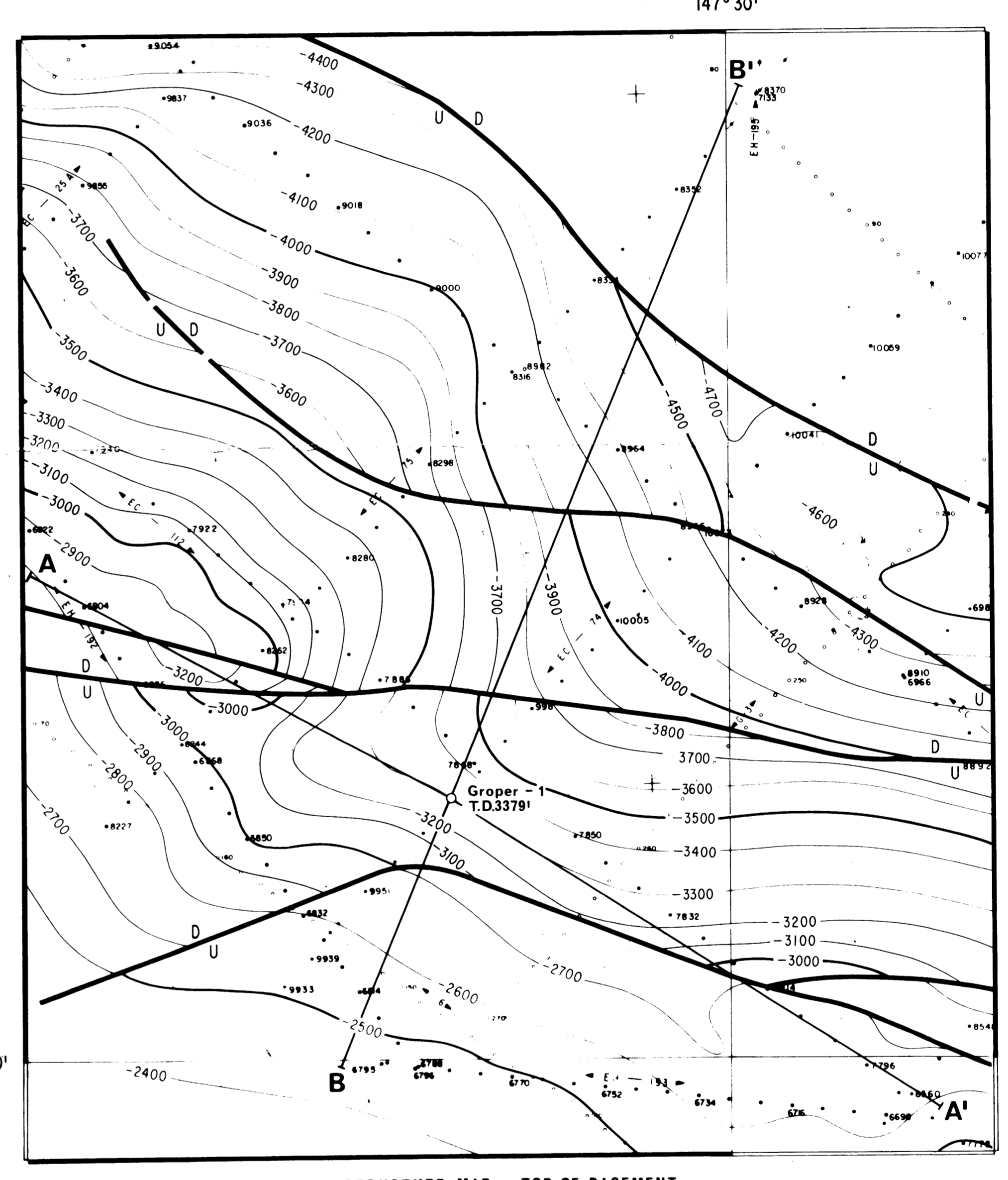
STRUCTURE MAP - TOP OF BASEMENT
