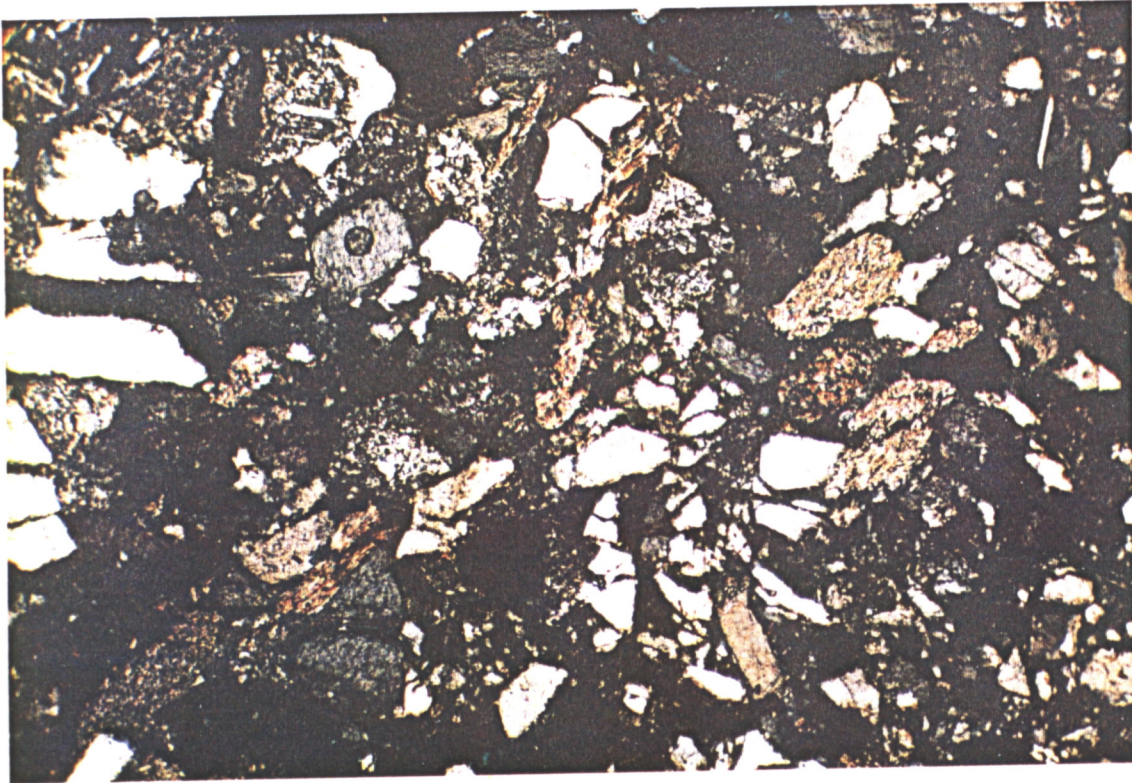
PHOTO 12 WIND. 2 3191M WELL SORTED LITHIC ARKOSIC ARENITE. NIC CROS. FIELD WIDTH 1.8MM
