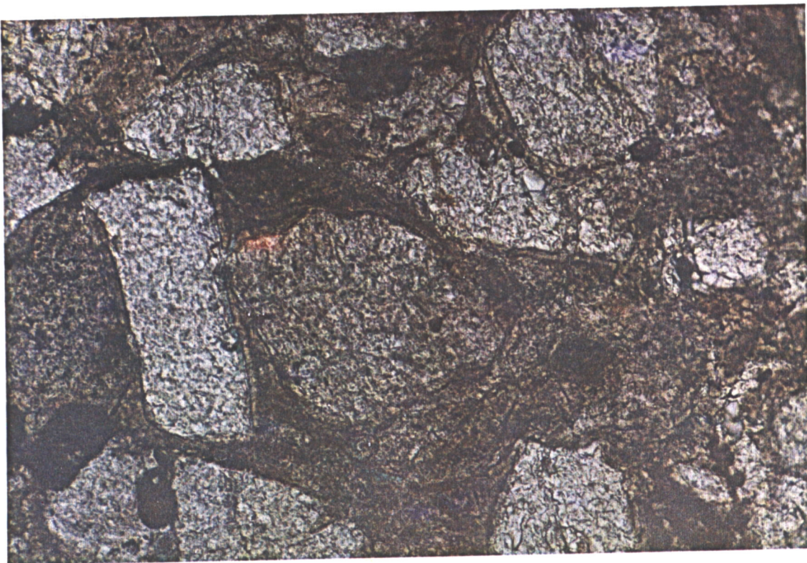
PHOTO 13 WIND. 2 3191M CLAY RIMMING ALL CLASTS AND FILLING PORES. NIC UNC. FIELD WIDTH 0.7MM
