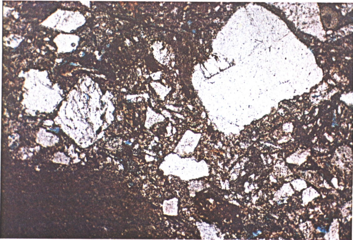
PHOTO 7 WIND. 2 1793M POORLY SORTED LITHIC ARKOSIC SANDSTONE/ GREYWACKE. NIC UNC. FIELD WIDTH 1.8MM
