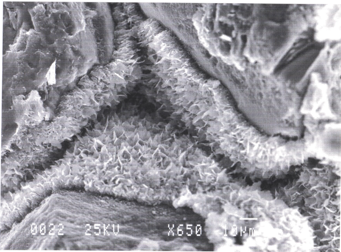
Figure 8: Sample 17: Plain light (upper) and SEM (lower) photomicrograph of chlorite pore lining within feldspathic litharenite. Long axis of upper photomicrograph is 0.62mm and scale bar in lower photomicrograph is 10 \mu m.
