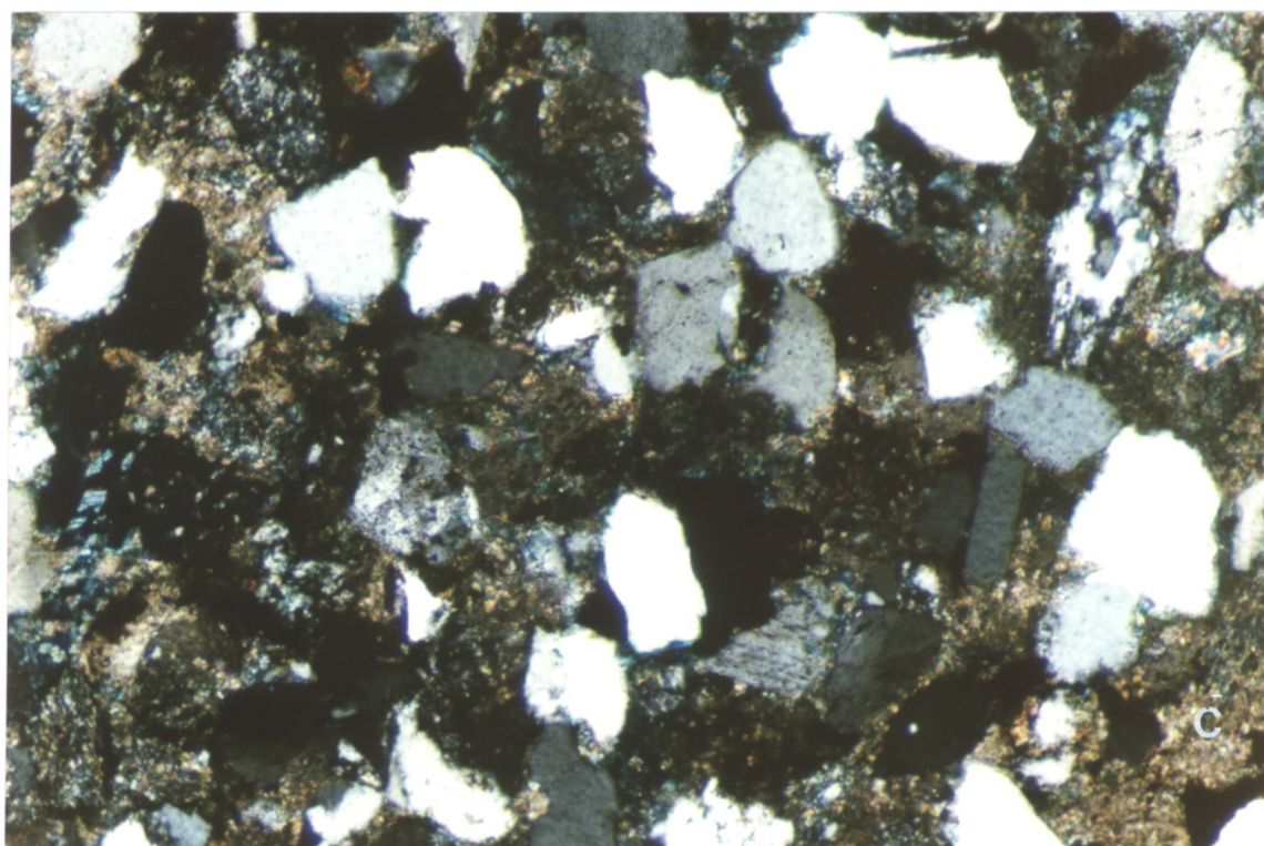
Figure 2: Sample 3: Plain light (upper) and cross-polarised (lower) photomicrograph of fine-grained, well sorted lithic arkose. Photomicrograph shows pervasive Fe-dolomite cement (C), pyrite (P) and oversized pore space containing partially corroded euhedral dolomite crystalloids (X). Long axis of photomicrographs is 1.25mm.
