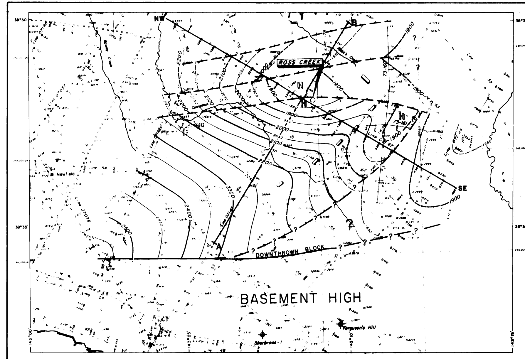
UNMIGRATED REFLECTION TIME CONTOURS INTRA - EUMERALLA
