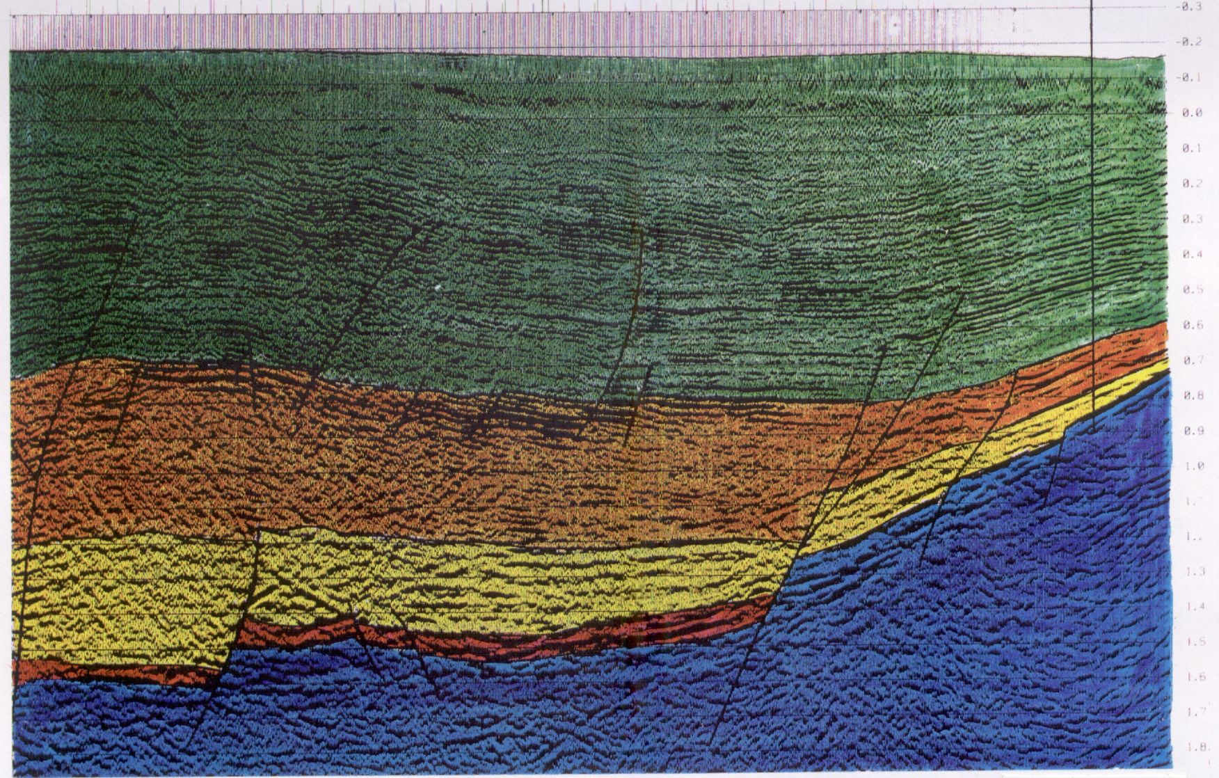
SEISMIC LINE CR88-01 SHOWING THE LOCATION OF MOCAMBORO No.11 STRATIGRAPHIC WELL ( SEISMIC LINE COURTESY OF BEACH PETROLEUM N.L. )
