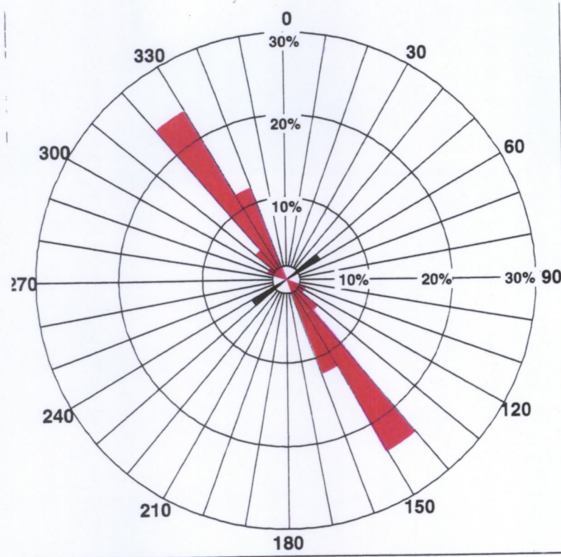
Figure G-1 Gordon-1 Borehole Breakout (black) and Drilling Induced Fracture (pink) strike plot. Mean strike orientation for Borehole Breakouts is 052°-232° and 144°-324° for Drilling Induced Fractures.
