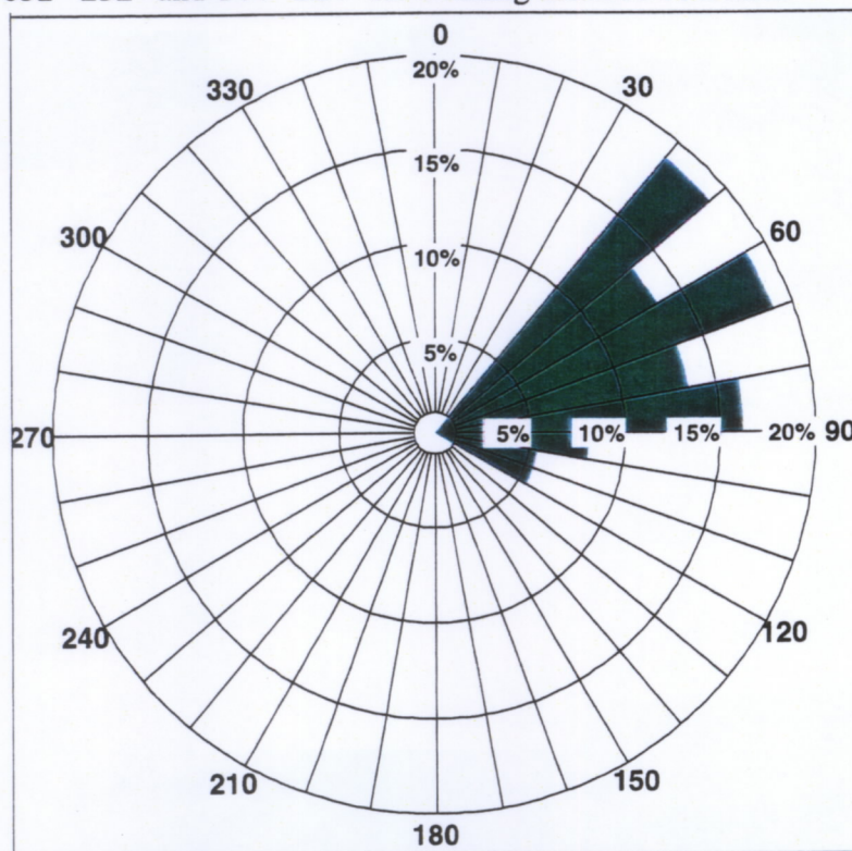
Figure G1-2 Gordon-1 Casterton Formation Shale bed boundary dip histogram. Mean dip orientation is 8.0°/071°.
