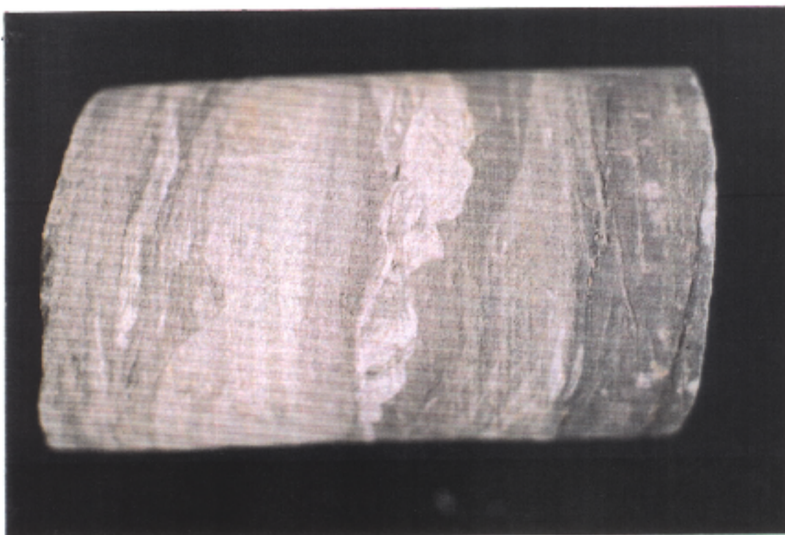
Detailed section of Core 3: Showing flame or squirt structures caused by loading of new sediment onto saturated clays and silts.
