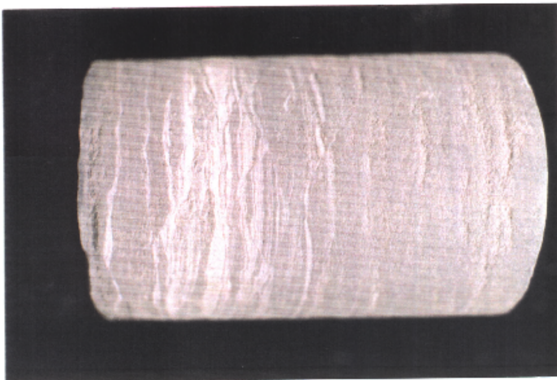
Detailed section of Core 3: This section of core, approximately 10cm long, shows wavy bedding and microfaulting in fine siltstone and sandstone layers.
