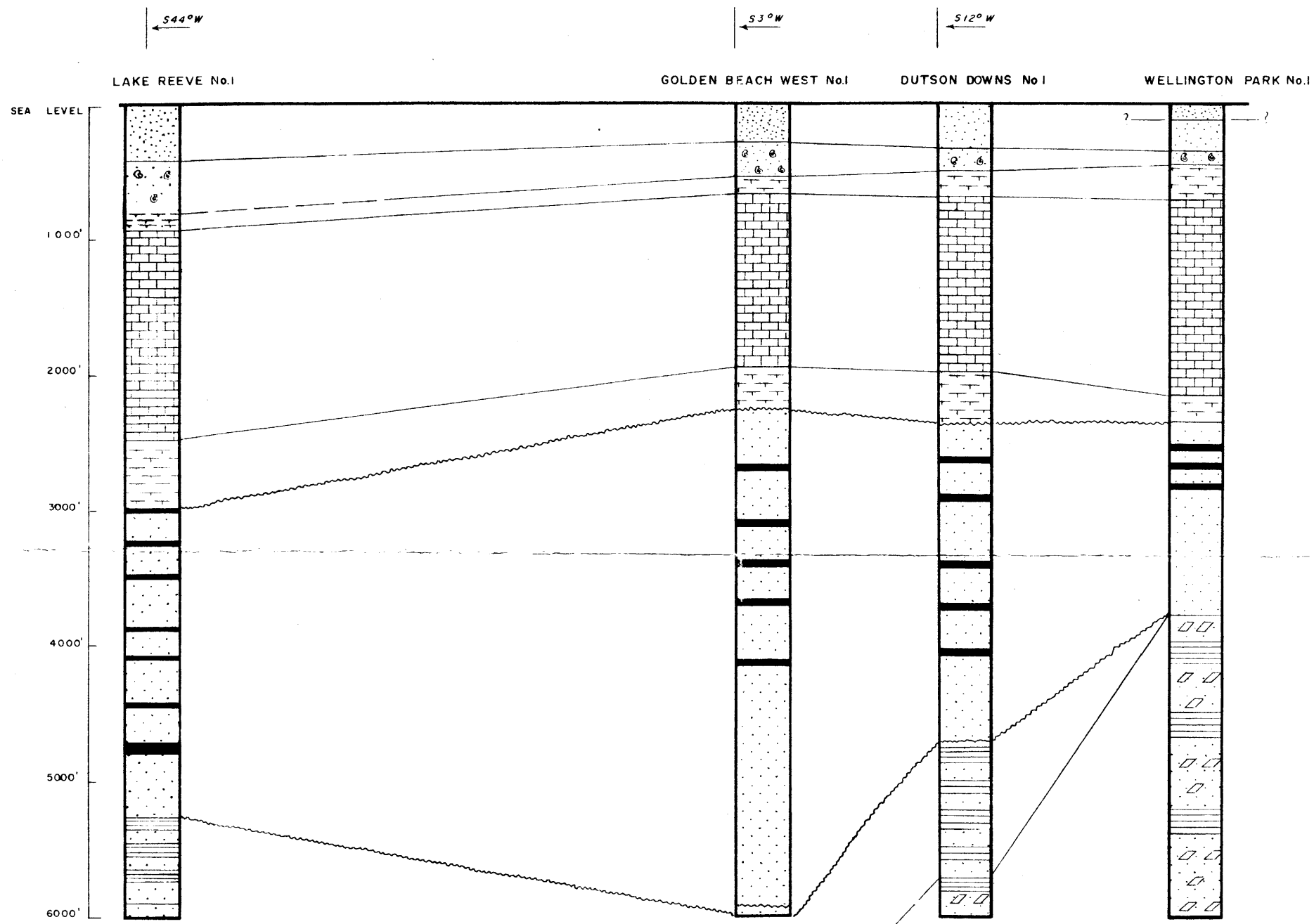
GEOLOGICAL SECTION BEFORE DRILLING
