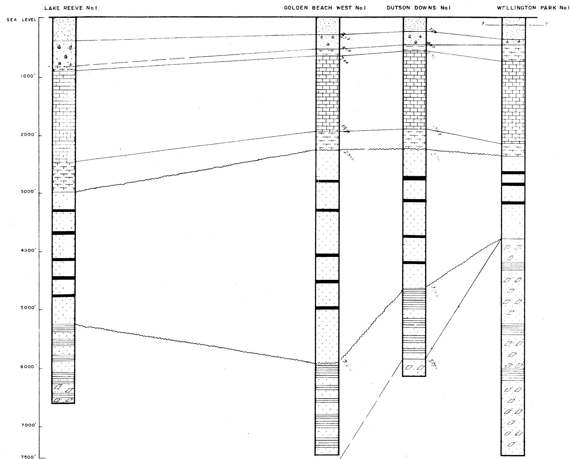
GEOLOGICAL SECTION AFTER DRILLING
