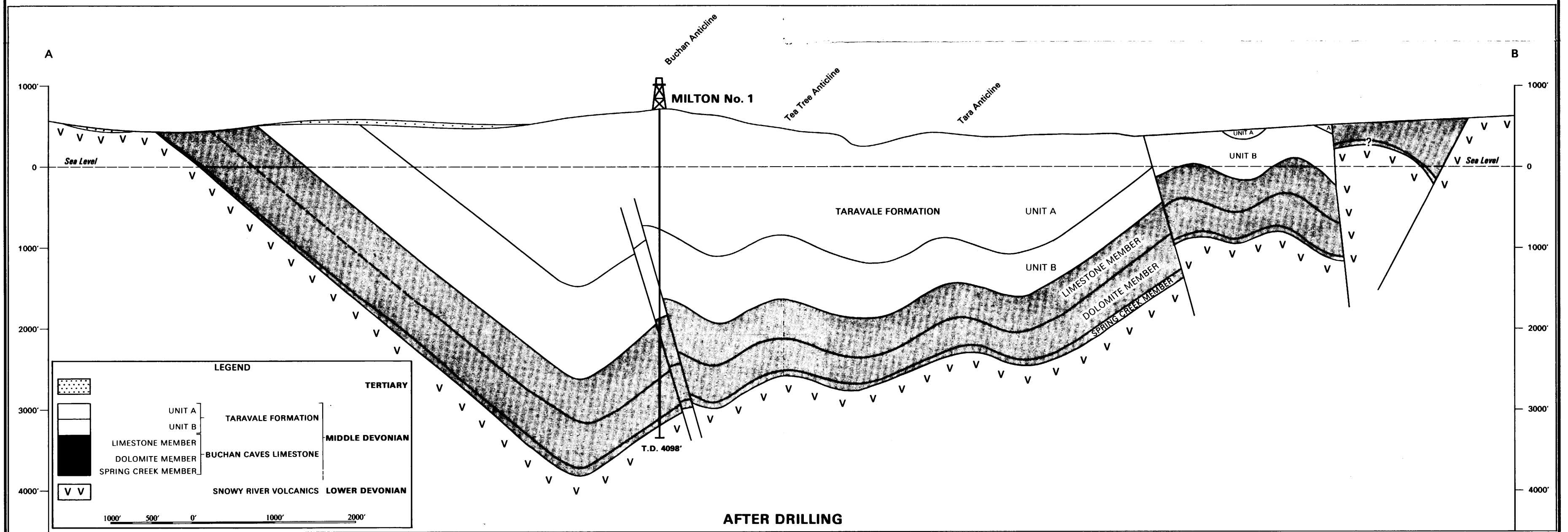
SECTION ACROSS BUCHAN SYNCLINORIUM BEFORE AND AFTER DRILLING
